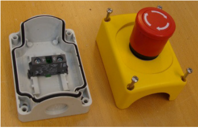
The emergency stop button used as the main scenario.
