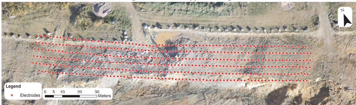
Figure 1. Aerial orthophoto of part of the rock quarry acquired approximately half a year after the geophysical investigations were performed. Positions of the electrodes used for the geoelectrical measurements are shown as red dots.
