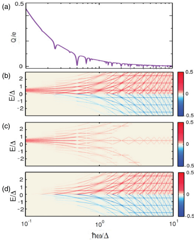
FIG. 4. (Color online) (a) High-frequency regime of the transferred charge Q per period, displaying dips at frequencies given by Eq. (23). (b)–(d) Energy distributions f_{\text{out}}(E) [in (b)], the bias contribution f_{\text{out}}^{\text{bias}}(E) [in (c)], and the pumping contribution f_{\text{out}}^{\text{pump}}(E) [in (d)] are shown. In all the plots T_A(t), T_B(t) as in Fig. 2 and kT \ll \Delta .
