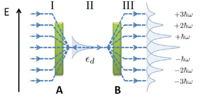
FIG. 3. (Color online) Schematic of the resonant paths in energy-position space, with three regions I, II, and III. In I electrons incident from terminal 1 pick up or lose a given number of Floquet quanta at contact A , to hit the resonance energy \epsilon_d . In II, the DB region between A and B , the electrons scatter elastically back and forth between the contacts. In III the electrons acquire 0, \pm 1 , \pm 2, \dots quanta when transmitting out through B .
