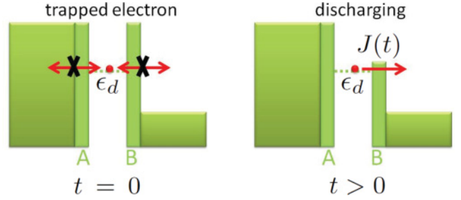
FIG. 6. (Color online) Sketch of the simplified model used to derive the single-particle wave function in the ideal regime. At t = 0 the electron is trapped between barriers, in a single level at energy \epsilon_d = 0 . For t > 0 the electron can start to tunnel to the right lead. The time-dependent lead-level coupling is J(t) .
