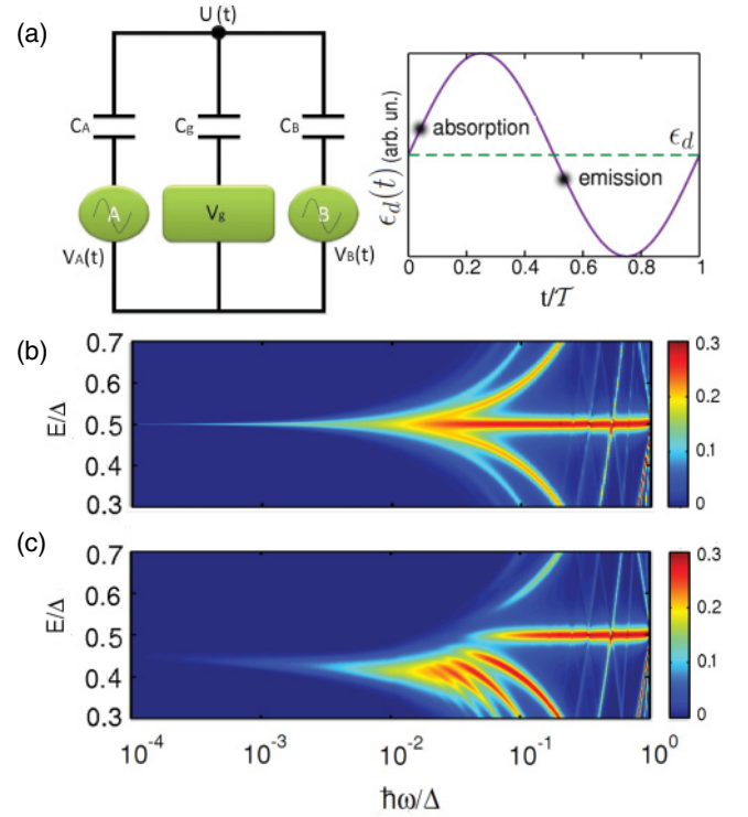
FIG. 7. (Color online) (a) Left: Circuit representation of the turnstile DB region capacitively coupled to quantum point contact gates A, B subjected to time-dependent bias V_{A/B}(t) and a top gate kept at constant bias V_g . Right: Sketch of the oscillation of the effective, instantaneous resonant level energy \epsilon_d(t) . Times for absorption and emission of the electron from the DB region for typical system parameters are shown with black dots. (b) Energy distribution f_{\text{out}}(E) for asymmetry factor e\alpha V^{\text{ac}} = 0 to compare with (c) f_{\text{out}}(E) for e\alpha V^{\text{ac}} = 0.1\Delta for a selected interval of E and \omega .
