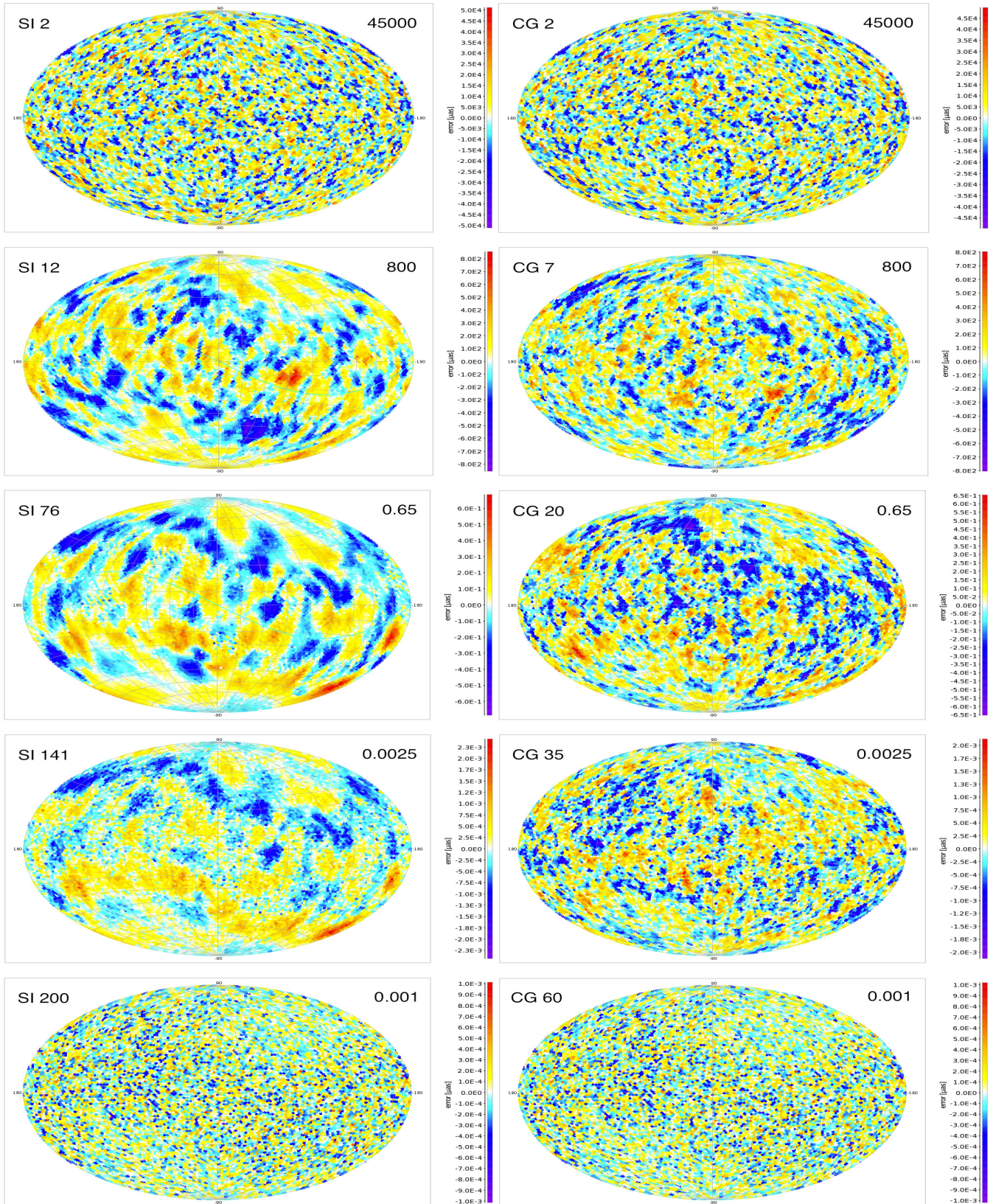
Fig. 2. Parallax error maps for test case A0 (no observation noise) at selected points in the simple iteration scheme (SI, left column) and conjugate gradient scheme (CG, right column). The iteration number is shown in the top left corner of each map (the initial values are iteration 2 due to the “start-up” procedure described in the text). The number in the top right corner is the approximate amplitude (in \mu\text{as} ) of the colour scale. Starting from identical initial values of the astrometric parameters, SI and CG converge to the same solution (equal to the true parallaxes to within \pm 0.001 \mu\text{as} ), although along different paths; moreover CG converges about four times quicker.
