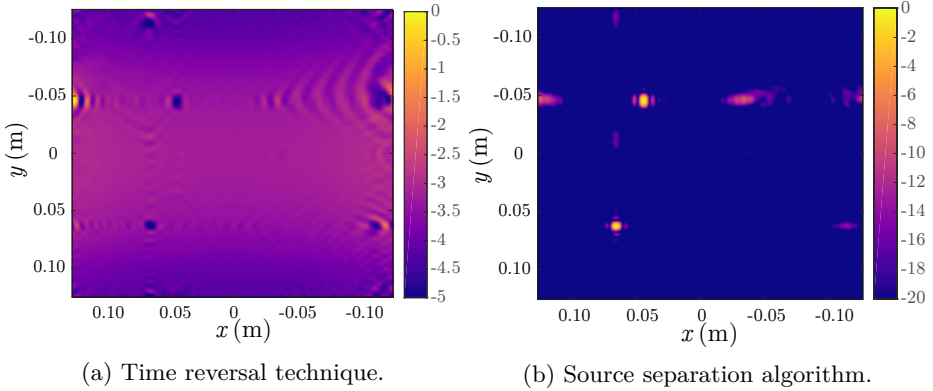
Figure 6: Retrieved images at 60 GHz for the synthetic data using the time reversal technique and source separation algorithm with customized color range. (a) depicts |E_y|/|E_y^{\text{FS}}| were |E_y^{\text{FS}}| denotes the free space reference measurement, and (b) depicts |E_y| . Both figures are in normalized dB-scale ( 20 \log_{10}(|u|/\max(|u|)) , where u is the parameter being plotted) with color range: (a) [-5, 0] dB, and (b) [-20, 0] dB.
