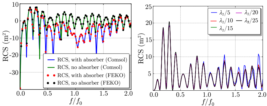
Figure 26: In the left plot the monostatic RCS of a capped cylinder simulated both in FEKO and in Comsol Multiphysics, with and without a Salisbury screen absorber, are presented. In the right figure a PEC capped cylinder scatterer has been simulated in Comsol Multiphysics using different mesh settings.
