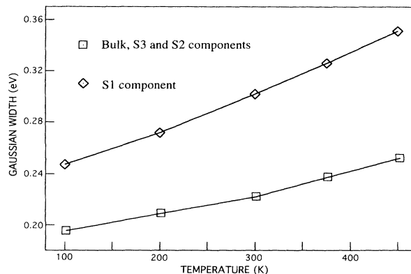
FIG. 4. Variation in Gaussian width (FWHM) with temperature, determined for the surface layer peak (S1) and for the other three components (B, S3, and S2), when an instrumental broadening of 80 meV has been removed by quadratic subtraction.
