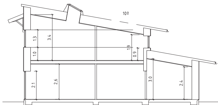
Figure 5.3 Section of Villa Malmborg (Drawing: Vårgårdahus).
