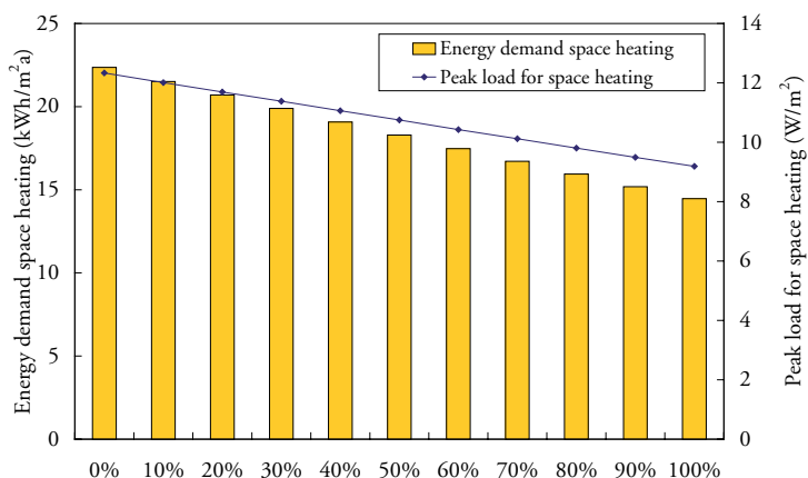
Figure 5.33 Energy demand for space heating ( \text{kWh/m}^2\text{a} ) and peak load for space heating ( \text{W/m}^2 ) at different heat exchanger efficiencies.
