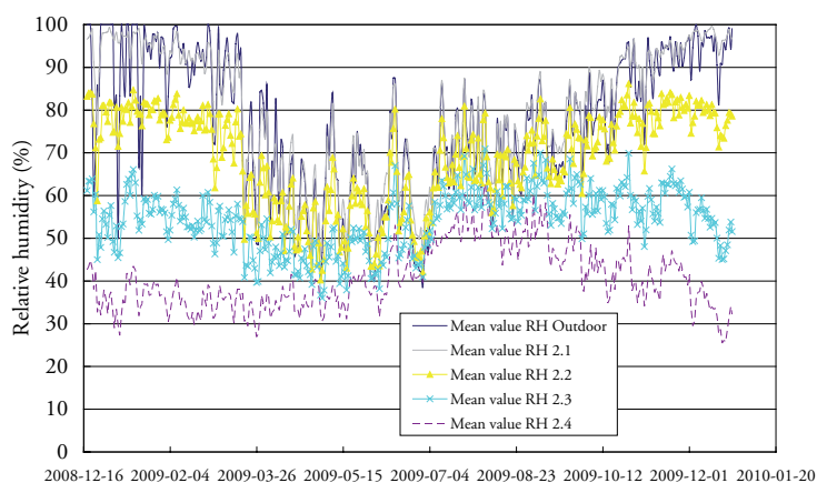
Figure 6.30 Daily Mean value of relative humidity in the four measuring points during the measuring period 081225 – 091225.
