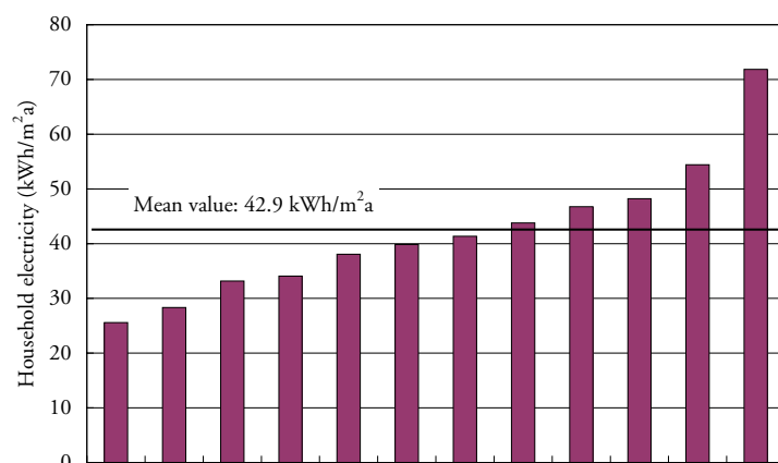
Figure 4.26 Use of household electricity during the period of 070201 – 080201.
