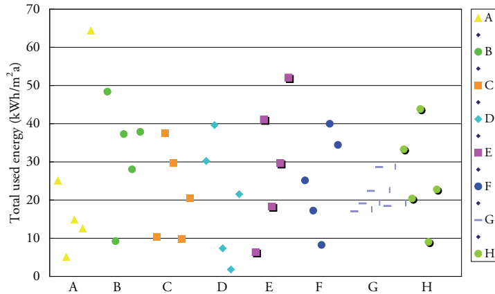
Figure 7.4 Total annual use of energy for domestic hot water for all 40 apartments, Värnamo during the period 070201 - 080201.
