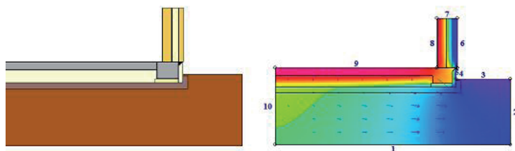
Figure 5.36 Thermal bridge simulation of foundation construction.
