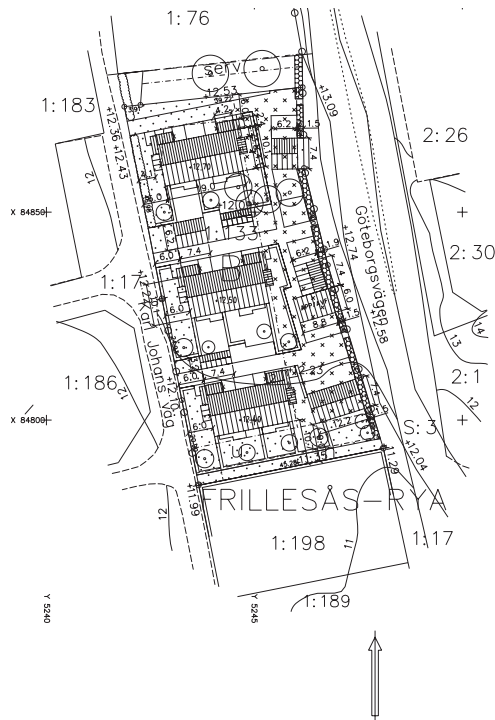
Figure 8.4 Site plan of the apartment buildings in Frillesås (Drawing: efem Arkitekter).
