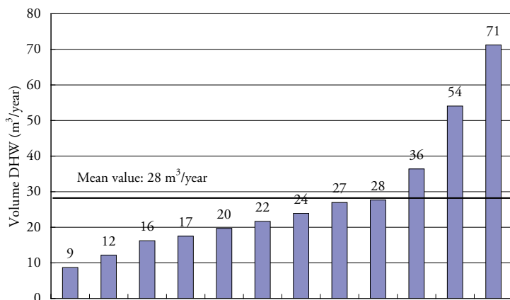
Figure 4.20 Measured volume of domestic hot water 070201 – 080201 (m³/year).
