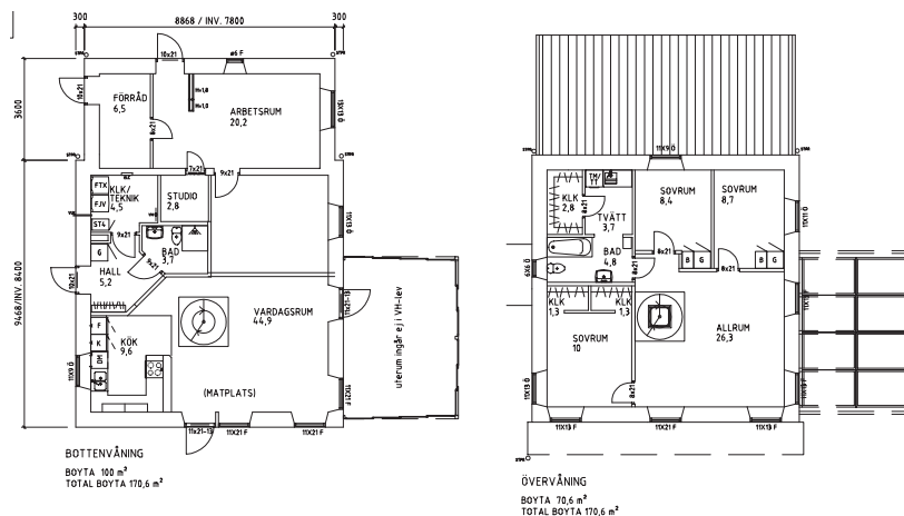
Figure 5.2 First and second storey of Villa Malmberg (Drawing: Vårgårdahus).
