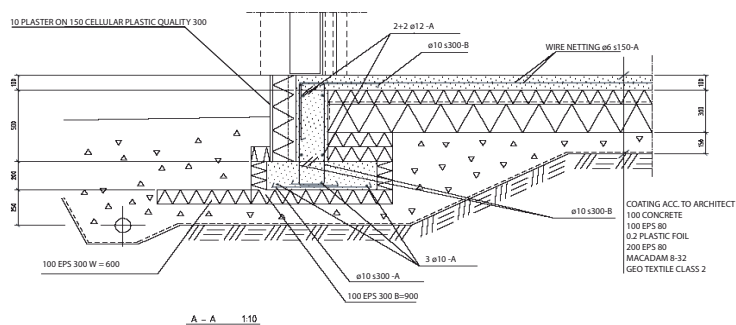
Figure 4.7 Foundation construction (Drawing: WSP Construction).
