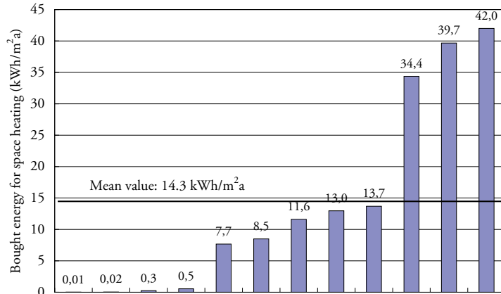
Figure 4.16 Bought energy for space heating during the period 071110 - 081110.
