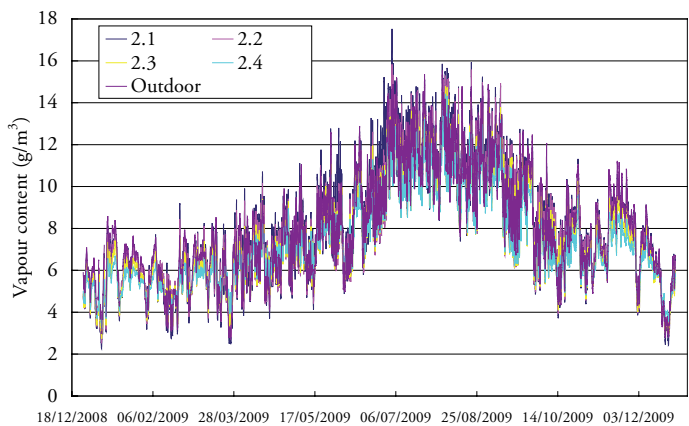
Figure 6.32 Calculated vapour content in the four measuring points and the outdoor reference point during the measuring period 081225 – 091225 based on all measured values.
