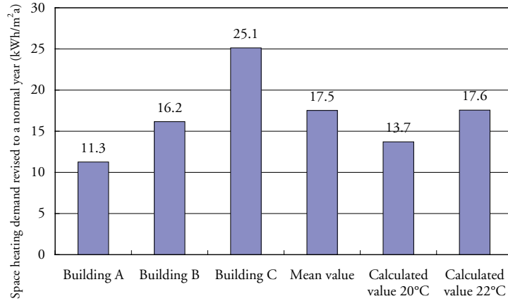
Figure 4.49 Measured and simulated energy demand for space heating revised to a normal year .
