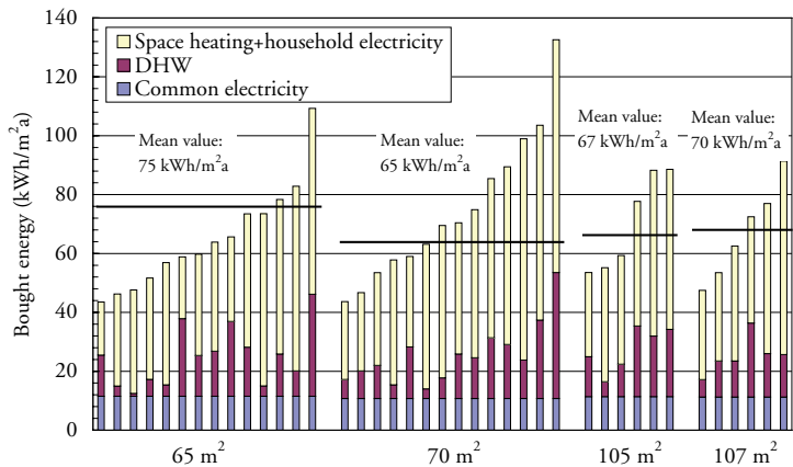
Figure 3.24 Bought energy for each apartment during the period 070201 to 080201, sorted by apartment size.
