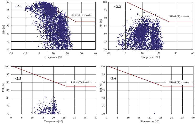
Figure 6.31 Relative humidity and temperatures in the four measuring points during the measuring period 081225 – 091222. Each point in the graph represents a mean measured value for one day and night (24h).
