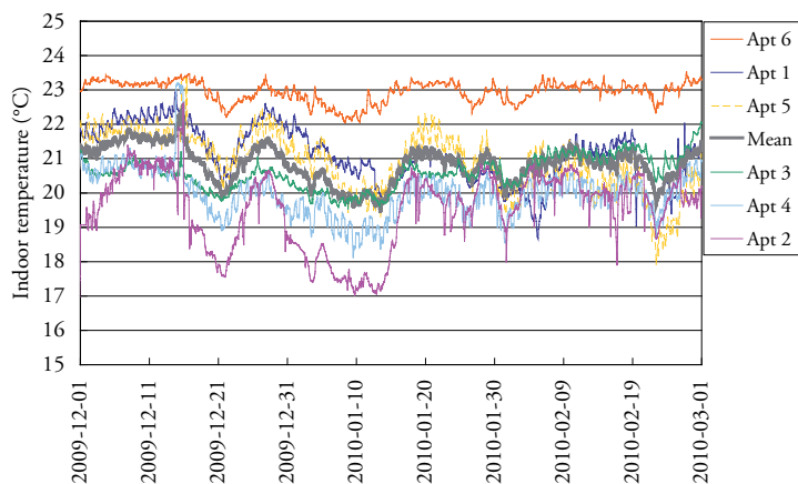
Figure 6.46 Measured indoor temperature in six apartments in Brogårdén 091201 - 100301.
