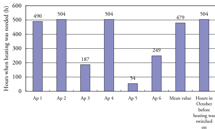
Figure 6.38 Number of hours when the indoor temperature was below 20 °C and additional space heating was needed in the six measured apartments together with the total number of hours before the heating distribution was switched on.
