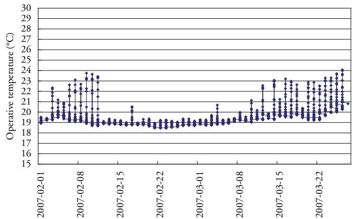
Figure 4.41 Mean value of measured operative temperature in the test apartment, 070201 - 070327.
