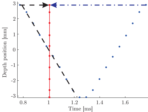
Figure 3.7: The measured depth positions of the laser sheet during a given period of scanning are represented by circles. The squares and the vertical line indicate the position and the target time for the interpolations. The arrows represents the interpolation process for one of the depth positions.
