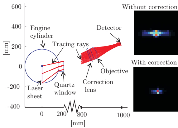
Figure 5.2: Ray-tracing of the laser-induced fluorescence imaged through a window with a curved inner surface. Three point sources are simulated, the insets showing the resulting images of one of these points, with and without use of the correction lens.
