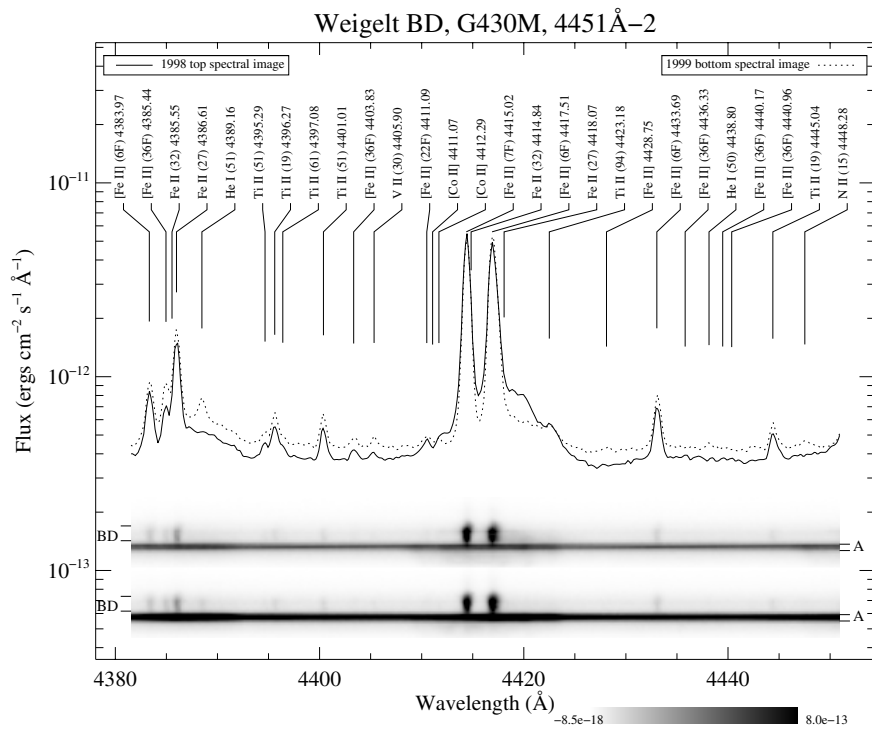
Fig. B.66. Spatially-resolved spectra of \eta Carinae, Weigelt B and Weigelt D. See Fig. 3 and text for detailed information.
