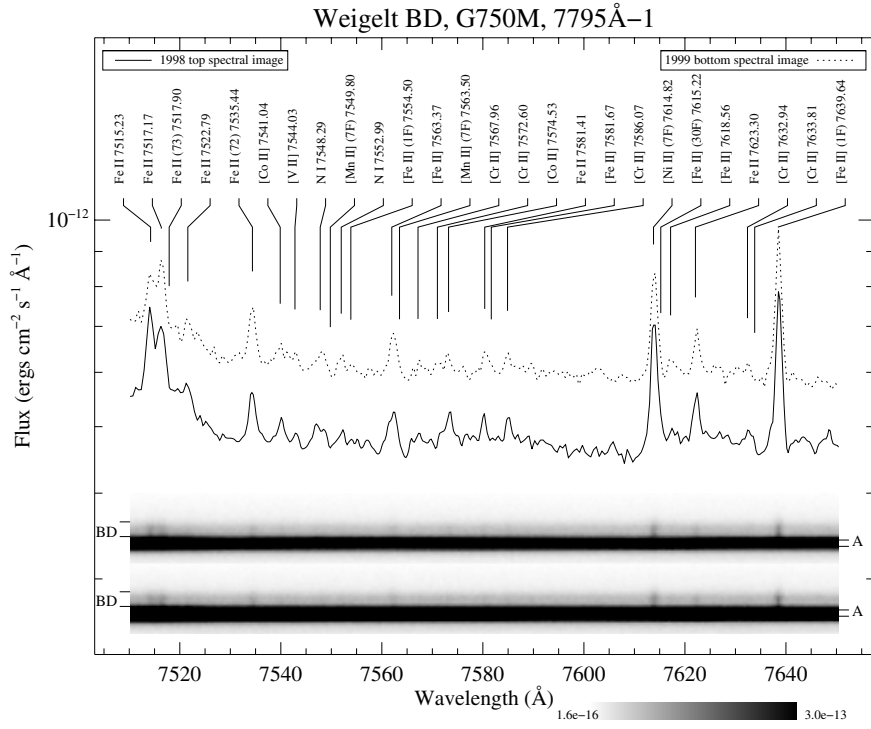
Fig. B.101. Spatially-resolved spectra of \eta Carinae, Weigelt B and Weigelt D. See Fig. 3 and text for detailed information.
