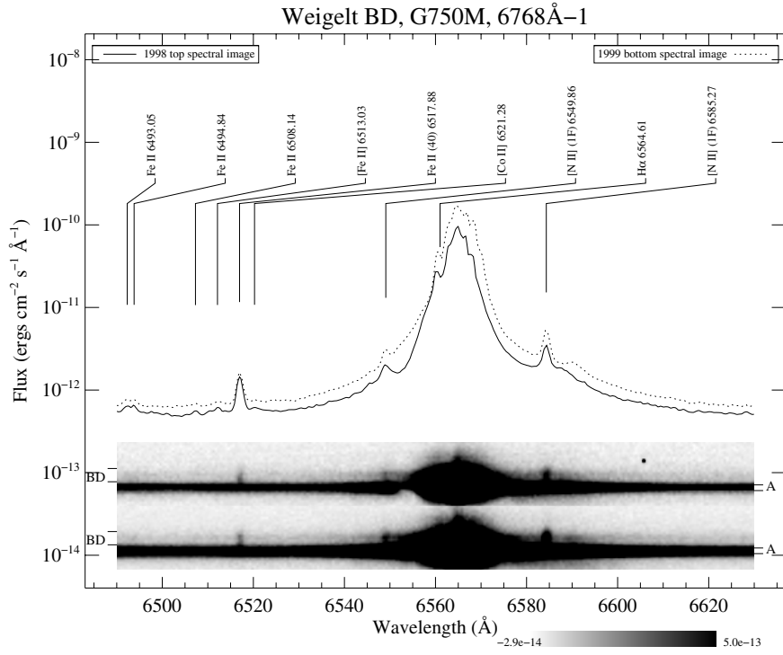
Fig. B.93. Spatially-resolved spectra of \eta Carinae, Weigelt B and Weigelt D. See Fig. 3 and text for detailed information.
