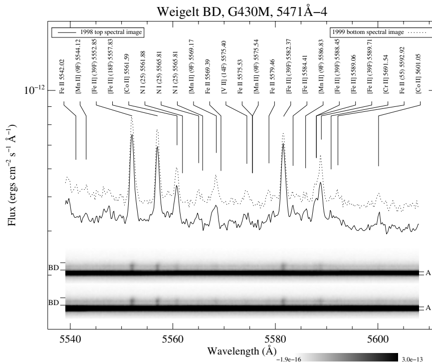
Fig. B.84. Spatially-resolved spectra of \eta Carinae, Weigelt B and Weigelt D. See Fig. 3 and text for detailed information.
