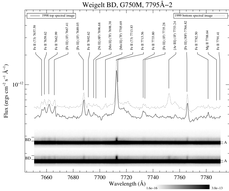
Fig. B.102. Spatially-resolved spectra of \eta Carinae, Weigelt B and Weigelt D. See Fig. 3 and text for detailed information.
