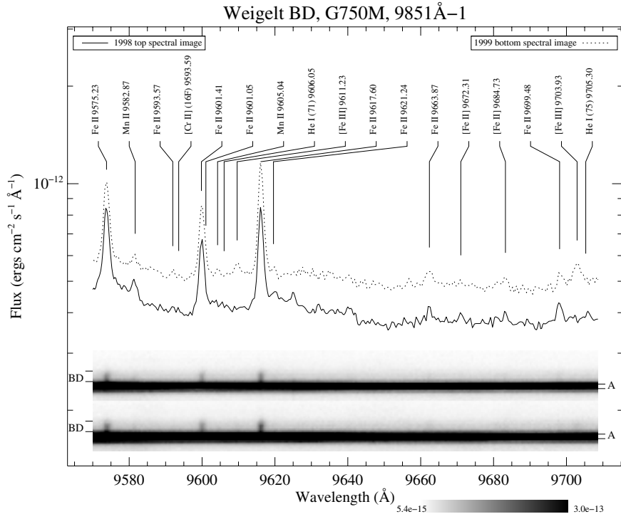
Fig. B.117. Spatially-resolved spectra of \eta Carinae, Weigelt B and Weigelt D. See Fig. 3 and text for detailed information.
