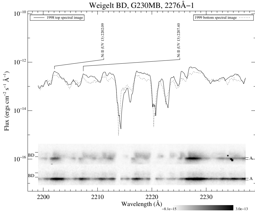
Fig. B.17. Spatially-resolved spectra of \eta Carinae, Weigelt B and Weigelt D. See Fig. 3 and text for detailed information.
