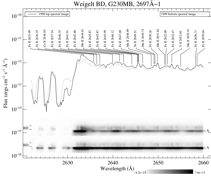
Fig. B.29. Spatially-resolved spectra of \eta Carinae, Weigelt B and Weigelt D. See Fig. 3 and text for detailed information.
