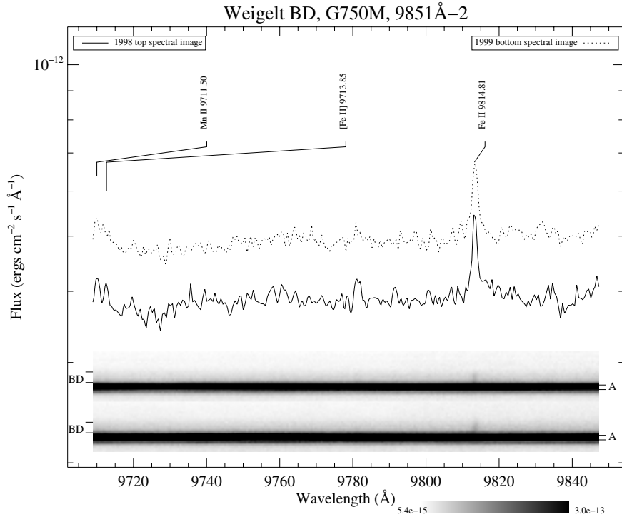
Fig. B.118. Spatially-resolved spectra of \eta Carinae, Weigelt B and Weigelt D. See Fig. 3 and text for detailed information.
