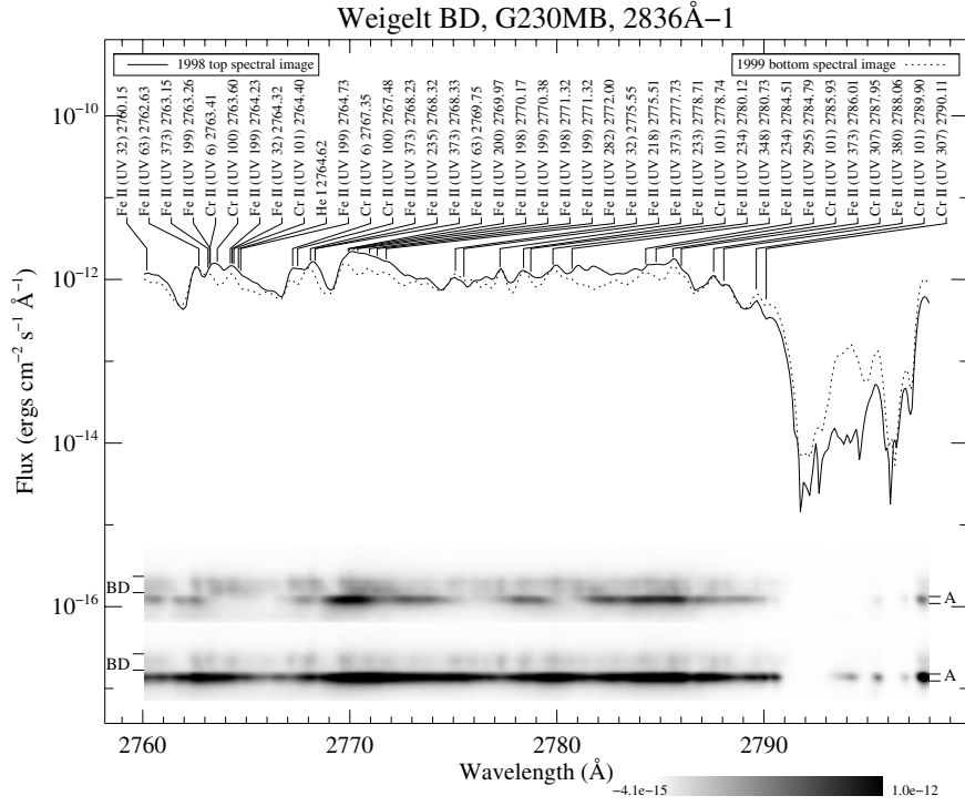
Fig. B.33. Spatially-resolved spectra of \eta Carinae, Weigelt B and Weigelt D. See Fig. 3 and text for detailed information.
