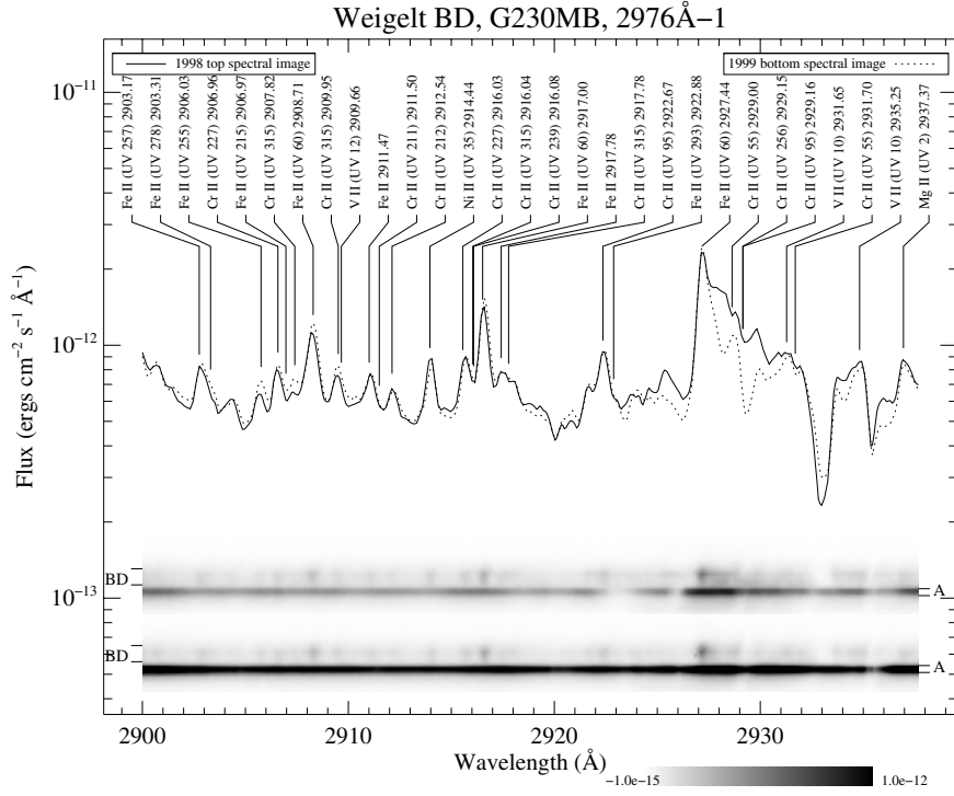
Fig. B.37. Spatially-resolved spectra of \eta Carinae, Weigelt B and Weigelt D. See Fig. 3 and text for detailed information.
