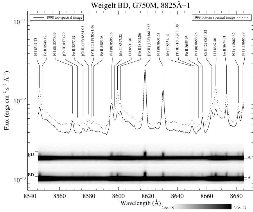
Fig. B.109. Spatially-resolved spectra of \eta Carinae, Weigelt B and Weigelt D. See Fig. 3 and text for detailed information.
