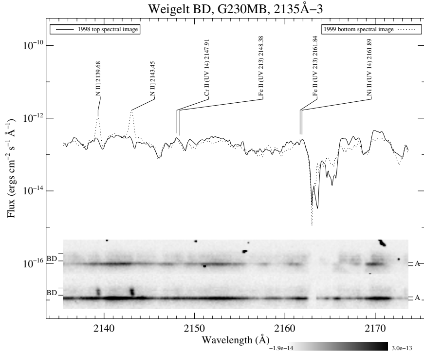
Fig. B.15. Spatially-resolved spectra of \eta Carinae, Weigelt B and Weigelt D. See Fig. 3 and text for detailed information.
