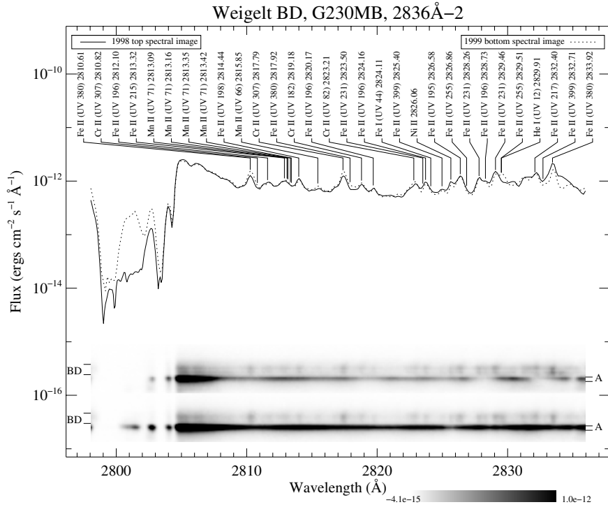
Fig. B.34. Spatially-resolved spectra of \eta Carinae, Weigelt B and Weigelt D. See Fig. 3 and text for detailed information.
