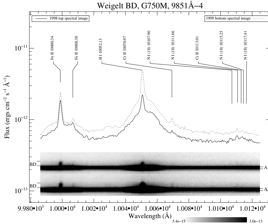
Fig. B.120. Spatially-resolved spectra of \eta Carinae, Weigelt B and Weigelt D. See Fig. 3 and text for detailed information.
