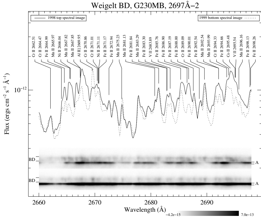
Fig. B.30. Spatially-resolved spectra of \eta Carinae, Weigelt B and Weigelt D. See Fig. 3 and text for detailed information.
