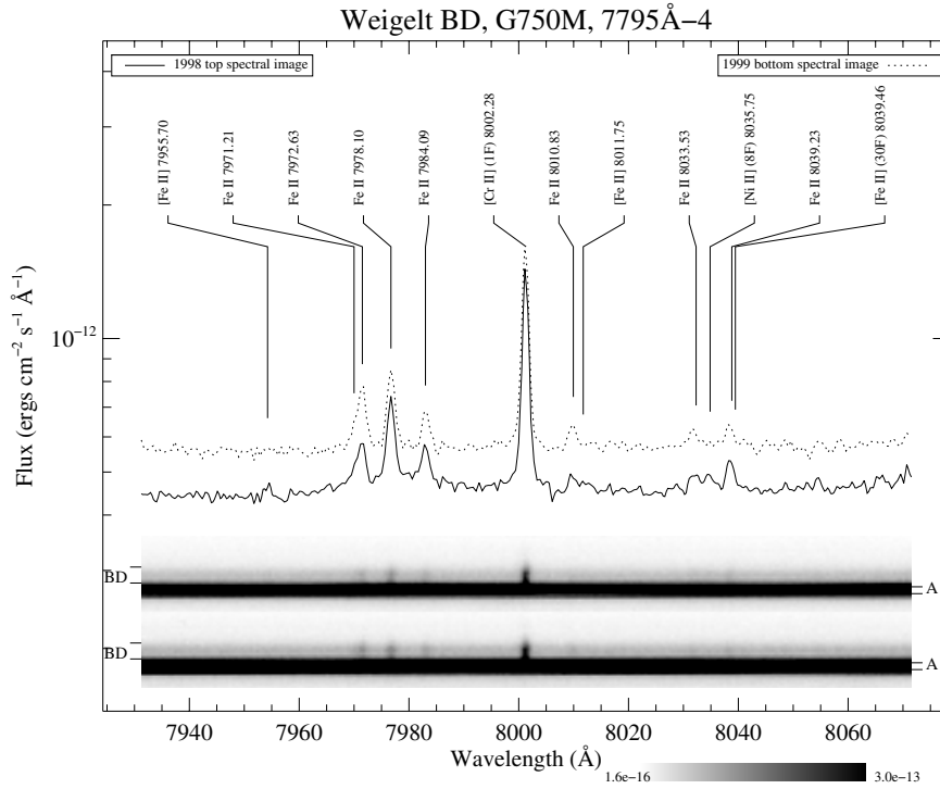
Fig. B.104. Spatially-resolved spectra of \eta Carinae, Weigelt B and Weigelt D. See Fig. 3 and text for detailed information.
