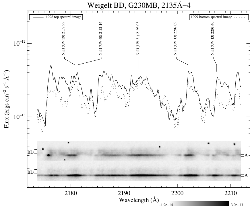
Fig. B.16. Spatially-resolved spectra of \eta Carinae, Weigelt B and Weigelt D. See Fig. 3 and text for detailed information.
