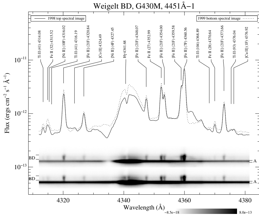
Fig. B.65. Spatially-resolved spectra of \eta Carinae, Weigelt B and Weigelt D. See Fig. 3 and text for detailed information.
