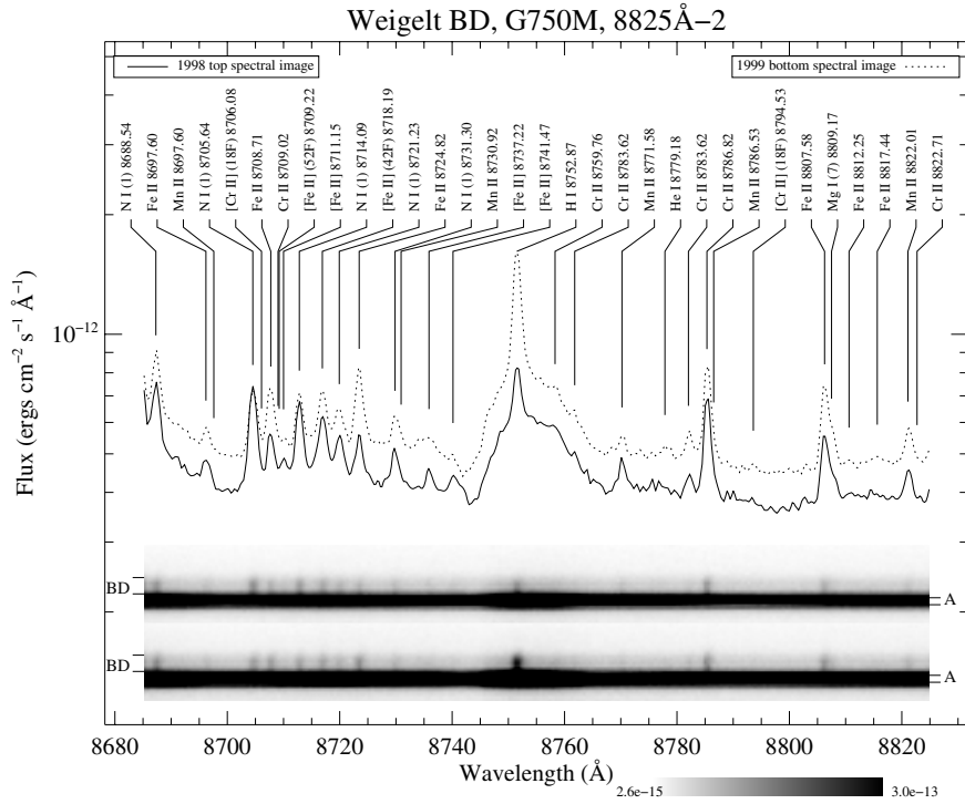
Fig. B.110. Spatially-resolved spectra of \eta Carinae, Weigelt B and Weigelt D. See Fig. 3 and text for detailed information.
