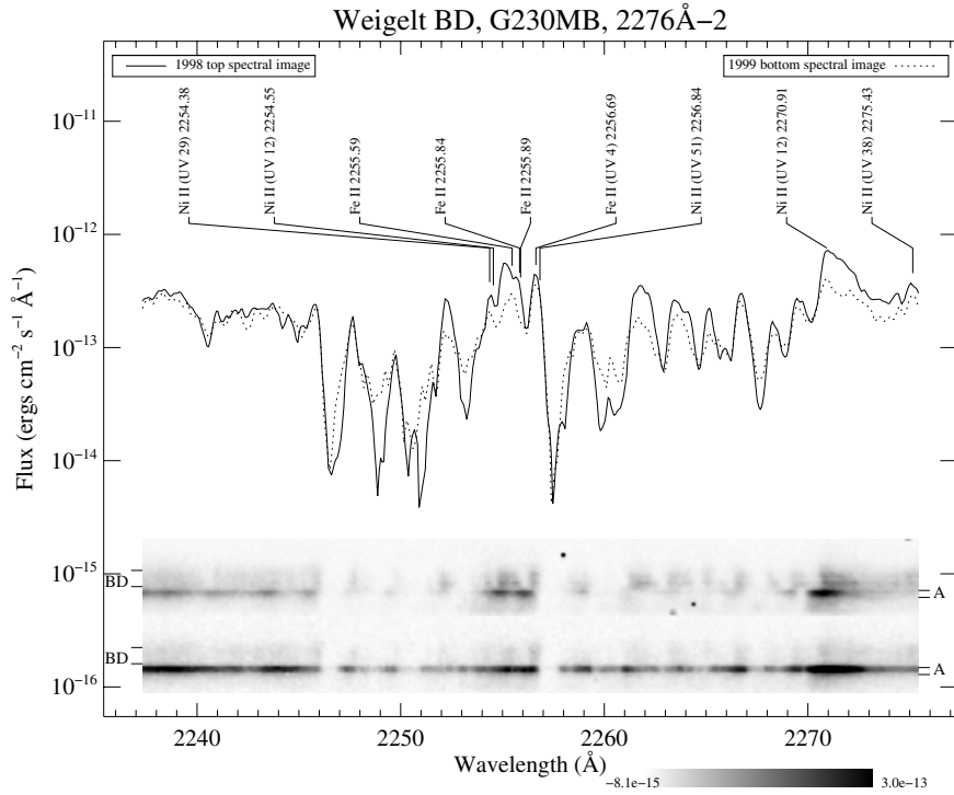
Fig. B.18. Spatially-resolved spectra of \eta Carinae, Weigelt B and Weigelt D. See Fig. 3 and text for detailed information.
