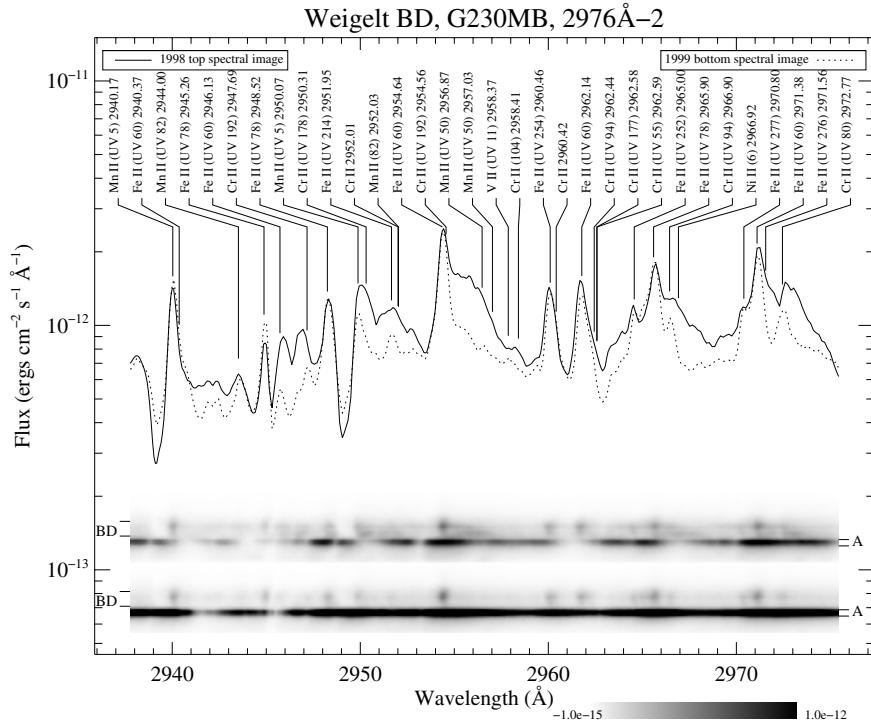
Fig. B.38. Spatially-resolved spectra of \eta Carinae, Weigelt B and Weigelt D. See Fig. 3 and text for detailed information.
