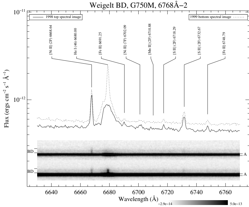
Fig. B.94. Spatially-resolved spectra of \eta Carinae, Weigelt B and Weigelt D. See Fig. 3 and text for detailed information.
