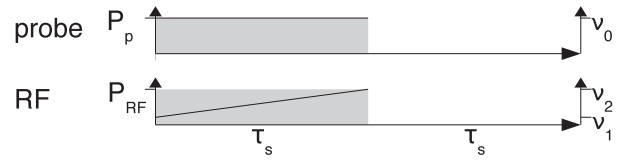
(b) Pulsed RHS, excited state experiments
