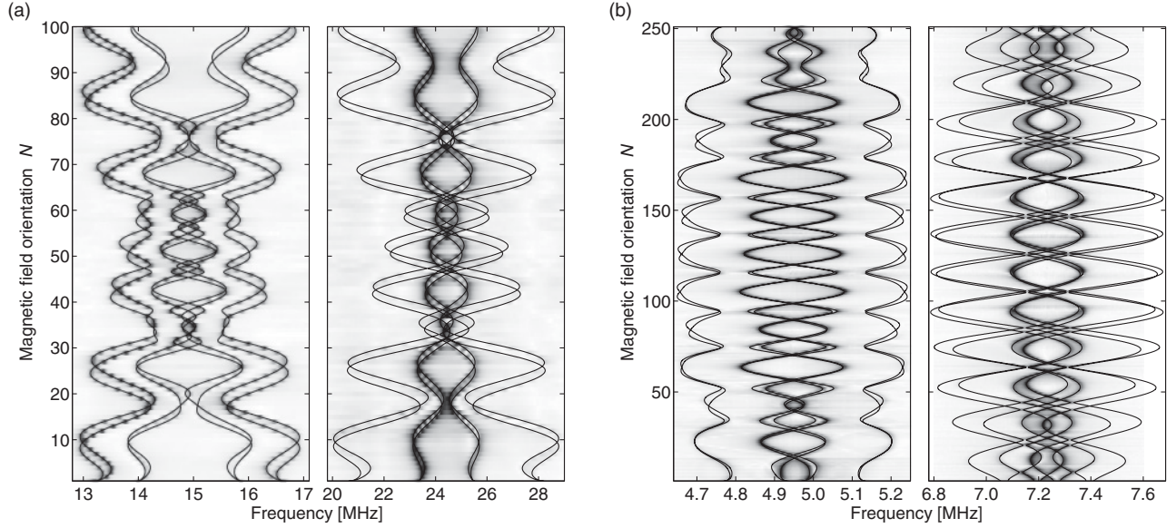
FIG. 4. RHS spectra of the |\pm\frac{1}{2}\rangle \leftrightarrow |\pm\frac{3}{2}\rangle and |\pm\frac{3}{2}\rangle \leftrightarrow |\pm\frac{5}{2}\rangle hyperfine transitions. (a) ^3H_4(0) ground-state cw RHS spectra. (b) ^1D_2(0) excited state pulsed RHS spectra. In both cases the solid lines represent the fit results and the shaded background the absolute value of the experimental spectra. For each field orientation, the spectrum was normalized to the maximum signal amplitude.
