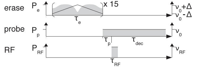
FIG. 2. RHS pulse sequences. Black lines indicate frequencies and gray areas the applied optical and rf powers. (a) Continuous-wave sequence for the ground-state measurements. A low-power laser probe ( P_p = 0.3 mW) and a scanning frequency rf ( P_{RF} \approx 1 W, \tau_s = 50 ms, \nu_1 = 7.4 , and \nu_2 = 22.4 MHz for |\pm\frac{1}{2}\rangle \leftrightarrow |\pm\frac{3}{2}\rangle or, respectively, 17.1 and 32.1 MHz for |\pm\frac{3}{2}\rangle \leftrightarrow |\pm\frac{5}{2}\rangle ) were applied to the sample. The optimum temperature of the cold finger for this scheme was 4.5 K, since still lower temperatures gave such slow hyperfine level relaxation rates that it would be necessary to repump the hyperfine level population. (b) Pulsed RHS sequence for the excited state. Probe and erase beam were overlapped in the sample at an angle of 0.6^\circ . To allow for higher repetition rate the chirped erase laser ( \Delta = 64 MHz, \tau_e = 10 ms, average power P_e \approx 20 mW) redistributed the populations. An initial population difference between hyperfine sublevels was created by the probe beam ( P_p = 1.2 mW, \tau_p = 100 \mu s) and converted to coherences by an rf pulse ( \nu_{RF} = 4.94/7.23 MHz ( |\pm\frac{1}{2}\rangle \leftrightarrow |\pm\frac{3}{2}\rangle resp. |\pm\frac{3}{2}\rangle \leftrightarrow |\pm\frac{5}{2}\rangle ), P_{RF} = 214/287 W, \tau_{RF} = 4 \mu s). For optical heterodyne detection the same probe beam was left active for an additional time \tau_{dec} . The temperature of the cold finger for this scheme was 2.4 K.
