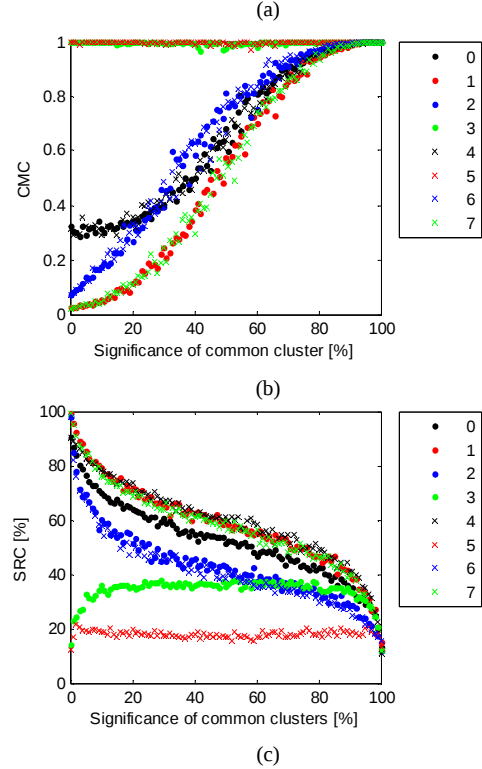
Fig. 2. Effect of common cluster simulated in controlled channels. (a) Simulation environment. (b) The correlation matrix collinearity (CMC), and (c) the relative sum rate capacity (SRC) as a function of the significance of common cluster. The legends show the correspondence between the curves and the locations of UCC1.
