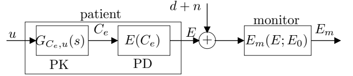
Fig. 2. Combined patient and monitor model with input u , measurement noise n , modeled surgical stimulation d , clinical effect E and measurement E_m .
