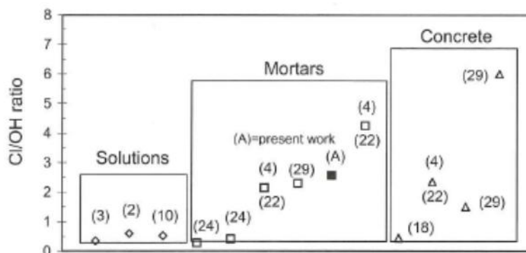
Figure 14. Chloride threshold values expressed as Cl/OH reported in the literature for alkaline solutions, mortars and concretes [61].
