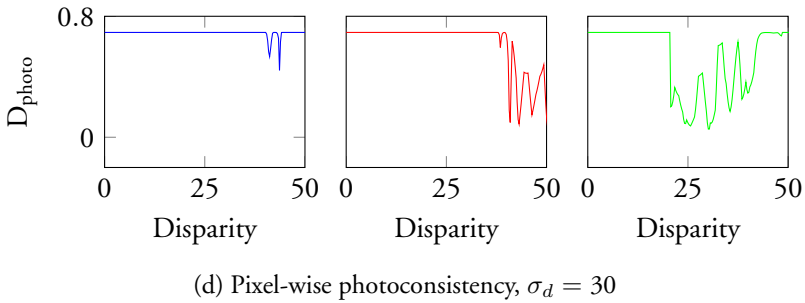
Figure 7.4: Comparing normalized cross correlation (NCC) to pixel-wise photoconsistency ( D_{\text{photo}} ) for a pair of stereo images. In the top row the two images are shown along with three color coded points. The two following rows show the resulting normalized cross correlation and pixel-wise photoconsistency for the three points.
