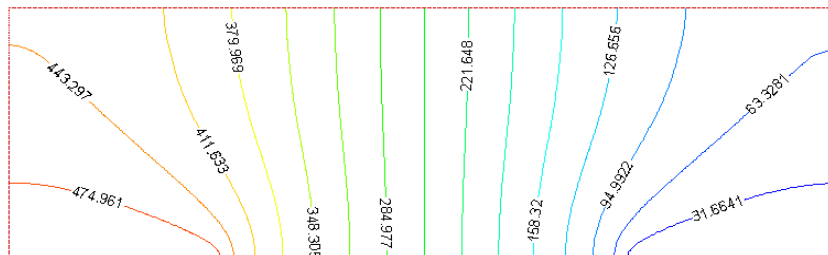
Figure 9: Pressure drop along the length of the cathode ( \text{N}/\text{m}^2 )
