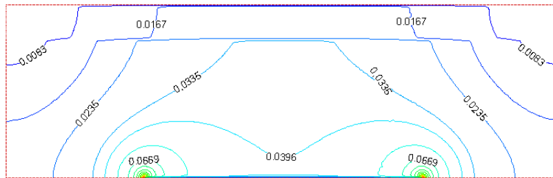
Figure 8: Velocity profile in the cathode of PEM fuel cell ( \text{m}/\text{s} )
