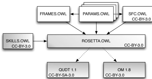
Figure 1: The original ontology structure, [18].
