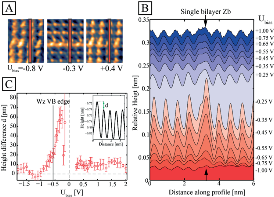
Figure 5.12. (A) STM images of single bilayer Zb segment in a Wz matrix, obtained on the \{110\}/\{11-20\} -type facets. I_{\text{set}} is 100 pA for all images. Red lines represent the position of line profiles used in (B) and (C). (B) Line profile across the stacking fault from STM images at different tip-sample voltages, V_T . (C) The difference in atomic corrugation, d , between the Zb atoms and the nearest Wz atom (as illustrated in inset) is plotted as a function of tip-sample voltage, V_T . Errorbars represent the standard deviation. Image adapted from Paper VI, [70].
