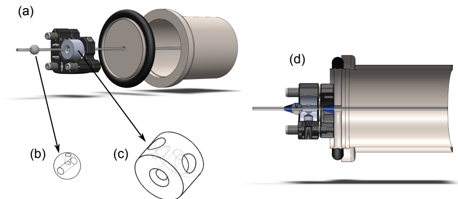
Figure A.8: Stretching device based on a standard 1/2'' optics mount glued to a KF40 blind flange with a central hole. a) View of the different components of the stretching device. b) Sketch of the plastic ball inside which the capillary is glued. c) Sketch of the aluminium cylinder that is fixed to the mirror mount with two M4 screws using the threaded holes on the side of the cylinder. The cylinder will push on the plastic ball to stretch the capillary when the alignment screws of the mirror mount are screwed in. d) Stretching device after it has been glued. The epoxy for fibre optics is shown in blue.
