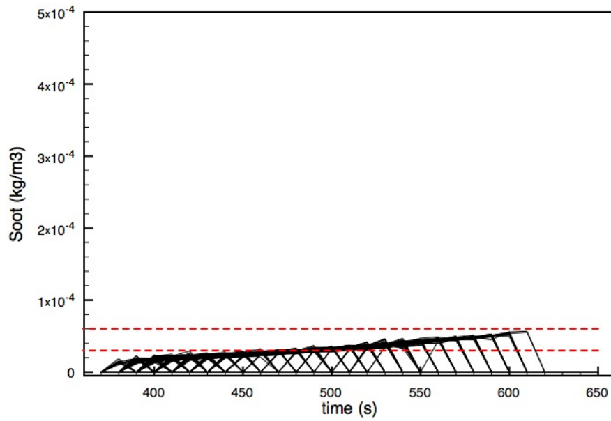
Figure 28. Soot concentration ( \text{kg}/\text{m}^3 ) for each person in the simulations for cable I
