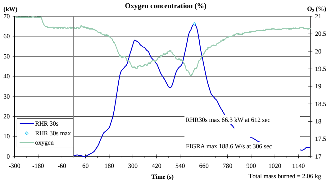
Figure 10. Heat release curves for cable I 2,3
