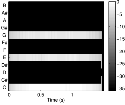
Fig. 5. The CEBS log-chromagram for the chord signal.
