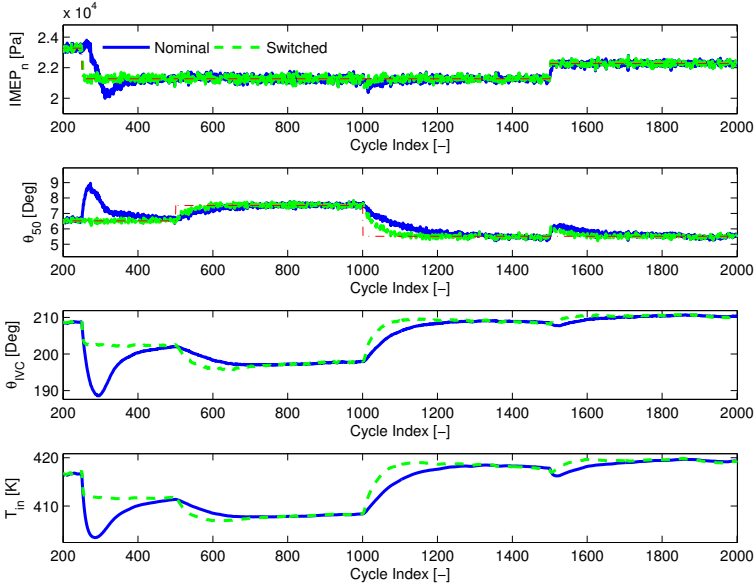
Figure 6.2 Simulated IMEP n , \theta_{50} , and control signals \theta_{IVC} and T_{in} for the nominal model predictive controller and the switched controller.
