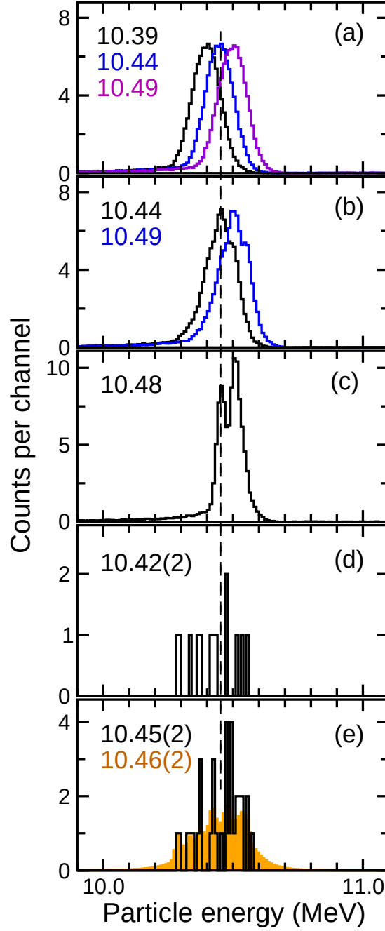
FIG. 2: Colour online: (a)-(c) Particle energy spectra resulting from various TASSISpec Monte-Carlo simulations [32] employing different Q_\alpha values and/or decay schemes of the decay of ^{288}\text{115} (cf. Fig. 3). (d) Experimental particle energy spectrum of the \alpha decay of ^{288}\text{115} [19]. (e) Experimental particle energy spectrum (black) and distribution (orange) of the \alpha decay of ^{288}\text{115} using combined data of Refs. [19–21]. The numbers in each panel reflect the mean value of the spectra in the interval [10.2,10.8] MeV. A dashed line at 10.45 MeV is indicated to guide the eye. The binning is 10 keV per channel. See text for more details.
