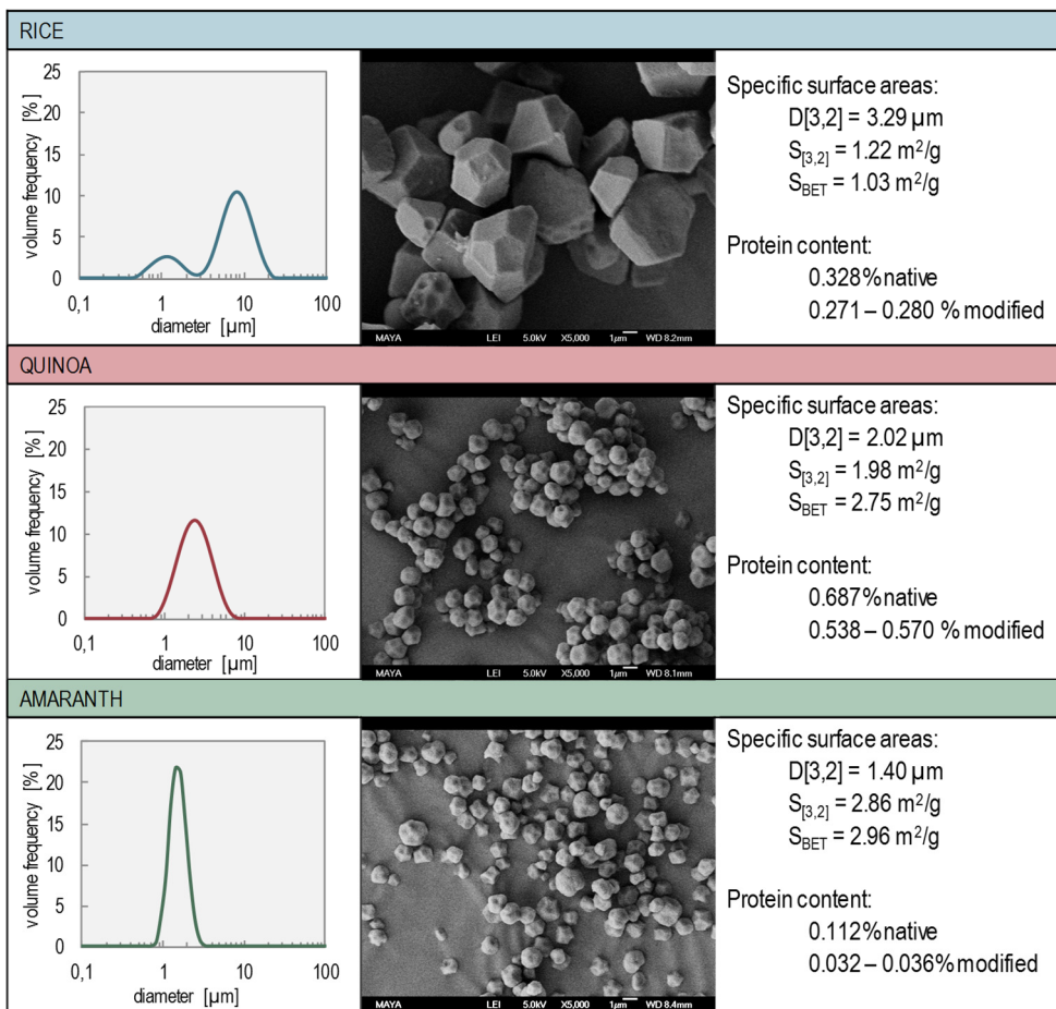
Fig 2. Particle size distributions, SEM images, specific surface data, and protein content of rice, quinoa and amaranth starches. Particle size data and images from Marefati, Wiege et al. 2017.
