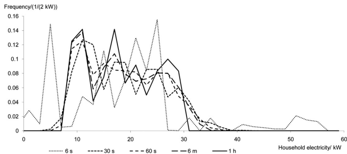
Fig. 5. The relative frequency of household electric power for different intervals ranging from 6 s to 1 h.
