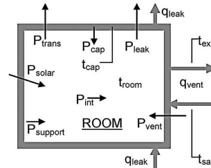
Figure 4. Power balance used in the simulation tool for the building. The air-handling unit is not shown and the energy going to it is not reported. Quantities are given in the text.
