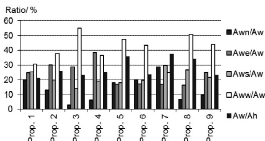
Figure 7. Window area per heated floor area and orientation of the window area in the properties.
