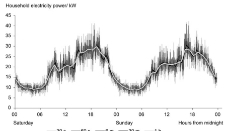
Fig. 3. The household electric power during Saturday through Sunday for different time intervals ranging from 30 s to 1 h.
