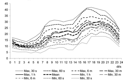
Fig. 4. The average household electric power for the measurement period presented for each clock hour of the day and the maximum and minimum at different intervals ranging from 30 s to 1 h. For example, the values at 8 are based on all data between 07 and 08 in the morning all the measured days. With 1 h resolution, it means one data per day, 5 in total, while it is much more data with 30 s resolution.
