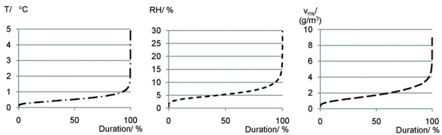
Figure 15 The duration of the daily span of temperature, T_{span} , relative humidity, \text{RH}_{span} , and moisture supply, v_{ms\_span} respectively. The presented values are average values of all locations.
