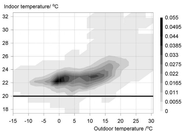
Figure 1. Relative frequency in the unit 1/(0.8^{\circ}\text{C} \cdot 2.4^{\circ}\text{C}) of indoor temperature and outdoor temperature for all the studied buildings, compared to EN 13788.
