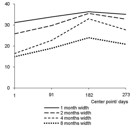
Figure 5. The annual space heating demand with internal heat load in pulses of pulse widths from 1 to 8 months, and at different centre points during the year according to Figure 1. The yearly internal heat load energy was the same for all pulse widths. A constant heat load with the same energy would result in a space heating demand of 18.1 kWh/m 2 .
