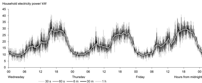
Fig. 2. The household electric power during Wednesday through Friday for different time intervals ranging from 30 s to 1 h.
