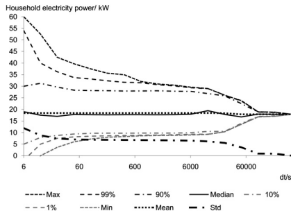
Fig. 1. Different statistical characteristics of the household electric power for intervals ranging from 6 s to 393,216 s in multiples of 6 s by 1, 2, 4, 8, ..., 65,536.
