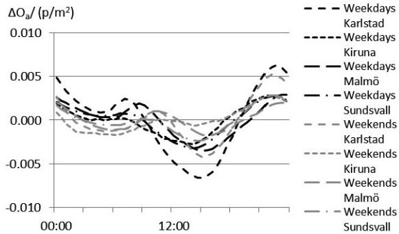
Figure 4. Variations in occupancy level during the day, presented for weekdays and weekends respectively. \Delta O_a is the average of (30 minute reading minus daily average). The values shown are average values of all buildings at a specific location.
