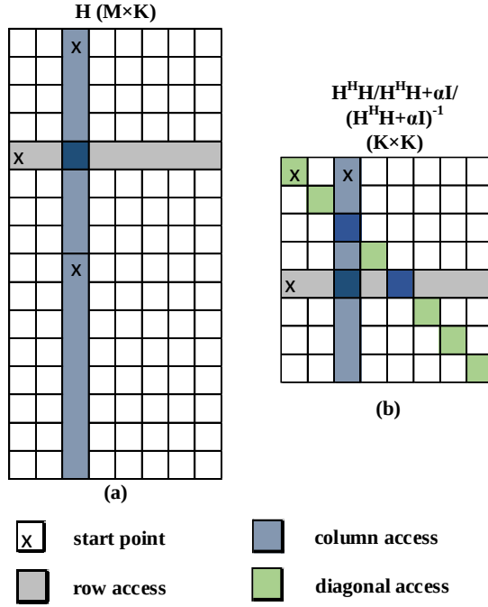
Figure 6.4. Examples of memory access patterns towards H and H^H H .
