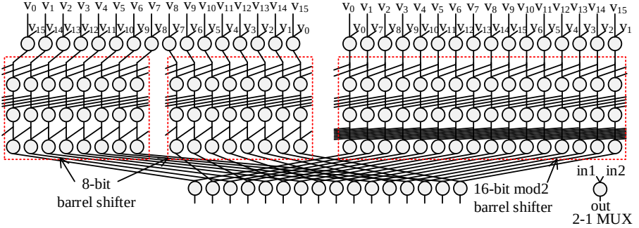
Figure 6.8. Permutation network.
