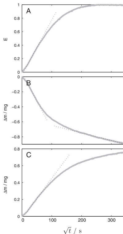
Fig. 2. Results from sorption measurements on a 2 mm thick sample of cement paste. A: example of a measured sorption curve with a similar shape as the Fickian curves in Fig. 1 (50–60% RH). B: example of a measured sorption curve that is bi-linear and distinctly non-Fickian (90–80% RH). C: example of a measured sorption curve that has an initial Fickian part, but that does not come to equilibrium as quickly as expected for a Fickian curve (60–70% RH). The dashed lines mark linear parts of the sorption curves.
