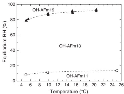
Fig. 20. OH-AFm19–OH-AFm13 and OH-AFm13–OH-AFm11 equilibria at 1 bar measured with the hydrate pair–humidity buffer method.
