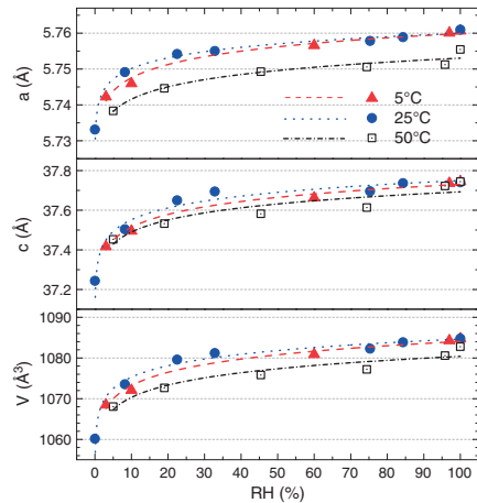
Fig. 13. Refined lattice parameters at 5 °C, 25 °C and 50 °C (sample at 0% RH was vacuum dried).
