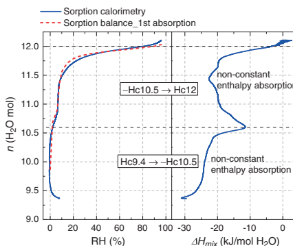
Fig. 11. Calculated sorption isotherm (left) and mixing enthalpy (right) of initially dry hemicarboaluminate at 25 °C from sorption calorimetry testing (for comparison the isotherm measured by sorption balance is superimposed in the left graph). Notice the two stepwise water uptakes and the variability of the mixing enthalpy during absorption.
