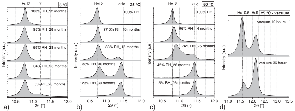
Fig. 7. XRD patterns of hemicarboaluminate dried at a) 5 °C, b) 25 °C and c) 50 °C at different RHs inside hermetic glass bottles, and d) vacuum dried at 25 °C during 12 h and 36 h.
