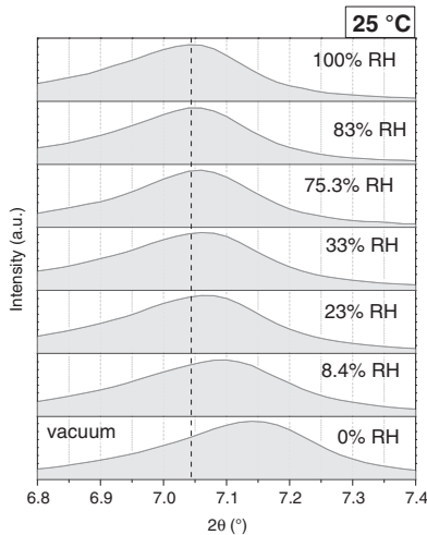
Fig. 12. XRD patterns of strätlingite dried at 25 °C and different RHs, showing the shift of the (0 0 1) reflection towards higher 2θ values (lower d -spacing). A similar trend was observed on samples aged at 5 °C and 50 °C.
