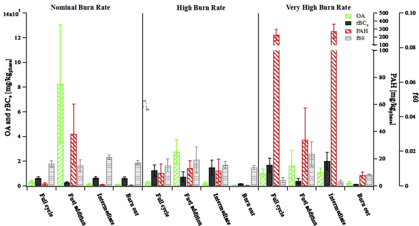
Fig. 3. Phase specific particulate emission factors of OA, rBC e , PAH together with the mass fraction of OA at m/z 60, f60 (C 2 H 4 O 2 + ), for nominal (NB), high (HB), and very high burn (VHB) rates in mg/kg phase based on 7, 6 and 3 cycles, respectively. The calculations are given for the three phases: fuel addition, intermediate and burn out. The full cycle emission factor (in mg/kg batch ) is given for comparison. Error bars represent the variation between the cycles and are given as the standard error of the mean.
