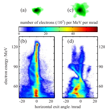
FIG. 2. (Color online) Effect of coma on the electron beam. [(a) and (b)] Flat wavefront, [(c) and (d)] coma = 0.175\lambda . (a) and (c) show the electron beam profile (average from several shots), (b) and (d) show the electron energy spectrum (from a single shot). The vertical axis is a linear energy scale and the horizontal scale represents the exit angle in the nondispersion plane.
