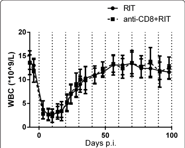
Figure 3 Myelosuppression after treatment. White blood cells in animals treated with RIT (solid line) and animals treated with anti-CD8 + RIT (dashed line). The error bars represent the standard deviation.
