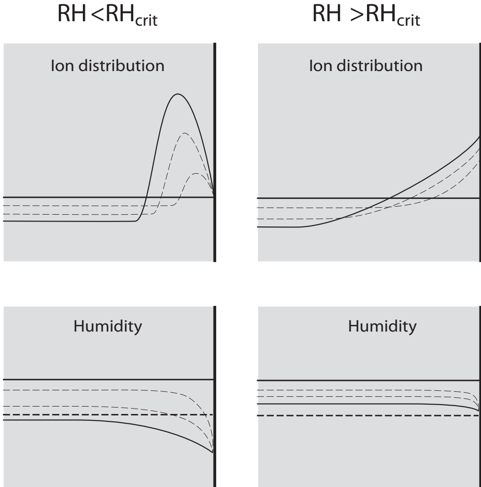
Figure 3.6: Redistributive ion distribution during drying at a surrounding humidity below (left) and above (right) the critical humidity (thick dashed line).
