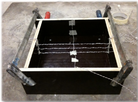
Fig 11. The mold and the thermocouples.
