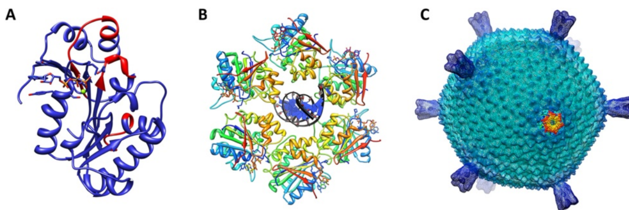
Figure 4 B204 structure. (A) Ribbon diagram of a B204 monomer bound to AMPPCP and Mg^{2+} (green sphere) (PDB: 4KFU) [7]. The regions highlighted in red indicate the conserved P9-motif described for the PRD1-like lineage of viruses [34]. (B) A hexamer model of B204 shown in rainbow hues (blue to red) generated by aligning six monomers of chain A of the AMPPCP B204 structure (PDB: 4KFU) onto each of the FtsK monomers in the FtsK hexamer (PDB: 2IUU) using the program UCSF Chimera [76]. According to our hypothesis the C-terminal part of B204 (orange to red) lies on the capsid distal side. A short stretch of dsDNA (black and blue helix) is modelled into the channel formed by the monomers. (C) A radially depth-cued isosurface representation (at 2 \sigma above the mean) of the 20-Å resolution reconstruction of STIV2 (EMDB: 1679) [71] with one of the turrets replaced by our hexameric model of B204 (surface representation in rainbow hues as in panel B). The figure was rendered in UCSF Chimera [76].
