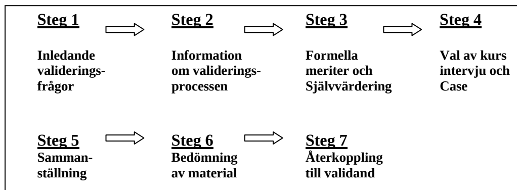
Figur 2. Valideringsmodell
