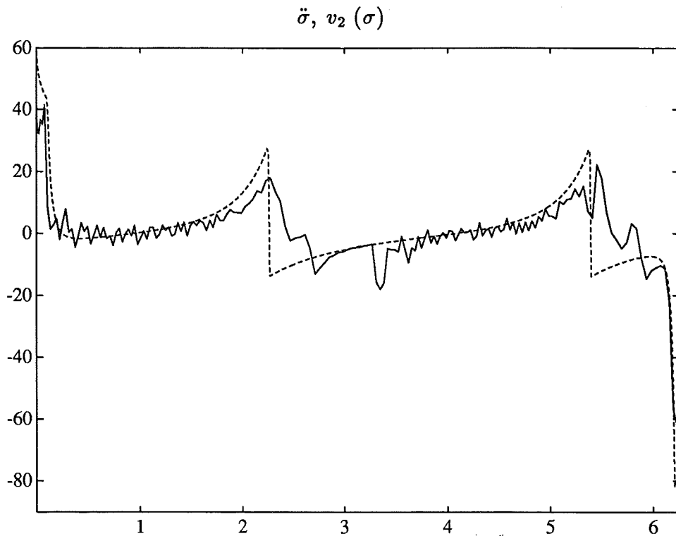
Figure 5.9 The nominal and actual path accelerations.
