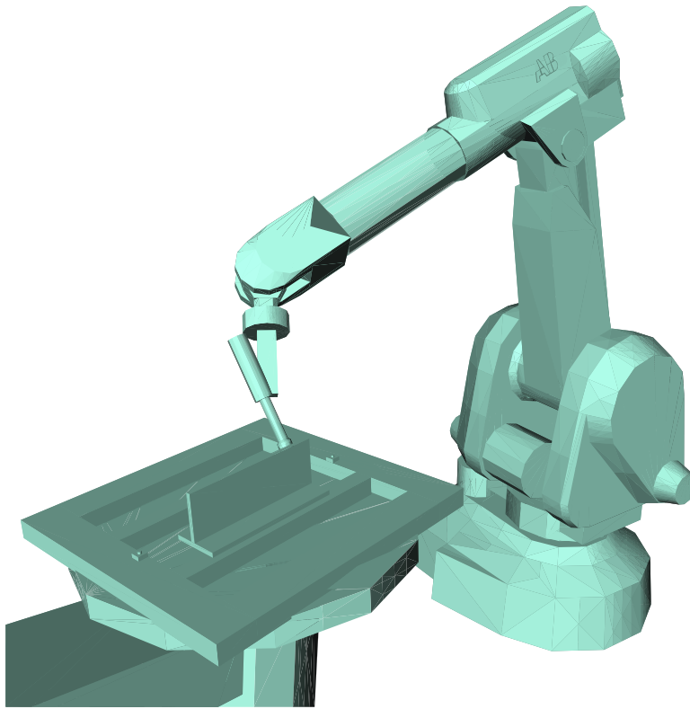
Figure 3.2 The simple welding application, using an ABB IRB-2000 robot, modeled in IGRIP [65].
