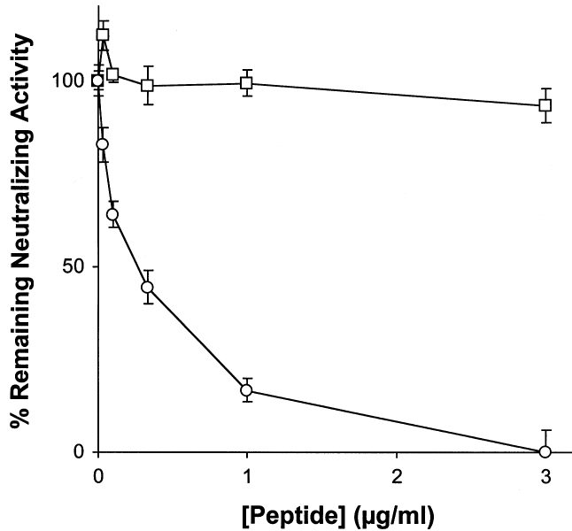
Fig. 2. Inhibition of the neutralizing activity of dimeric scFv by the addition of a soluble AD-2-mimicking peptide (O), or a negative control peptide (□). Experiments for all data points were performed in triplicate. The error bars indicate SEM.
