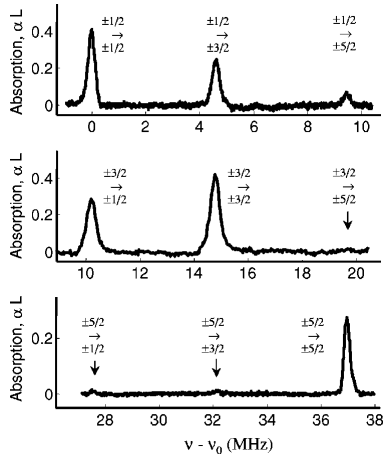
FIG. 7. Ions absorbing on specific hyperfine transitions, inside the inhomogeneously broadened {}^3H_4 - {}^1D_2 transition in \text{Pr}^{3+}:\text{Y}_2\text{SiO}_5 . The three curves correspond to three separate experiments. The three peaks of varying size, in each curve, are due to the same ensemble of ions absorbing on different transitions. The intensity was attenuated by a factor 10^3 during readout, in order not to cause significant excitation when probing the transitions. The scan rate during readout was of the order of r \approx 0.1 \text{ MHz}/\mu\text{s} . Single-shot measurements.
