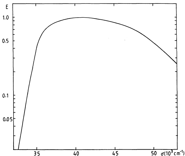
FIG. 1.—Efficiency curve for the Fourier-transform spectrometer derived from branching ratios in Ar II emitted by a hollow-cathode lamp.
