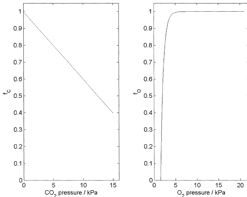
Figure 22: Factors f_C and f_O used for simulation of S. lacrymans behavior. The factors f_C and f_O take into account the influence of CO 2 and O 2 pressure on the activity of a sample
