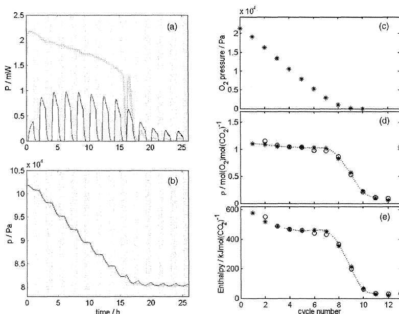
Fig. 2. Result of measurement with P. roqueforti growing on malt extract agar. The gray fields show when the valve is closed: (a) thermal power from P. roqueforti (gray line) and \text{CO}_2 absorbent (black line); (b) pressure changes measured in sample ampoule (gray line) and \text{CO}_2 absorbent (black line); (c) \text{O}_2 pressure; (d) metabolic gas exchange ratio calculated using Eq. (2) (stars) and Eq. (7) (circles); (e) metabolic enthalpy change calculated using Eq. (2) (circles) and Eq. (7) (stars).
