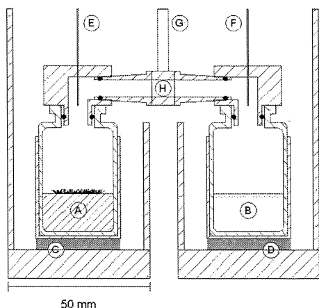
Fig. 1. A schematic drawing of the calorimetric device presented in the paper. A: Sample (agar with mould); B: CO 2 absorbent solution; C: sample calorimeter heat flow sensor; D: absorbent solution calorimeter heat flow sensor; E: sample ampoule pressure sensor tube; F: absorbent ampoule pressure sensor tube; G: shaft to turn valve; H: valve. Note that the drawing does not show the bottom parts of the heat sinks or the top part of the instrument with pressure sensors and step motor for valve operation. The instrument is placed in a thermostat.
