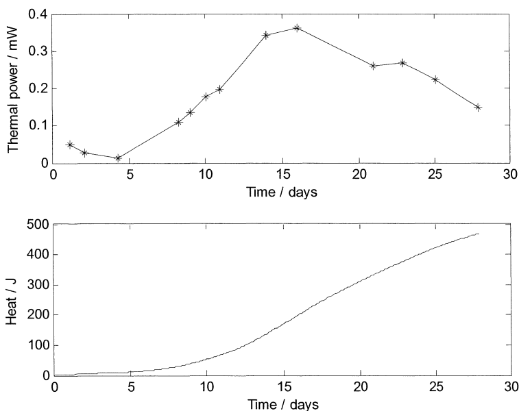
Figure 26: S. lacrymans (sample No. 15) thermal activities on MEA and the total heat production calculated by integrating the linearly interpolated top curve
