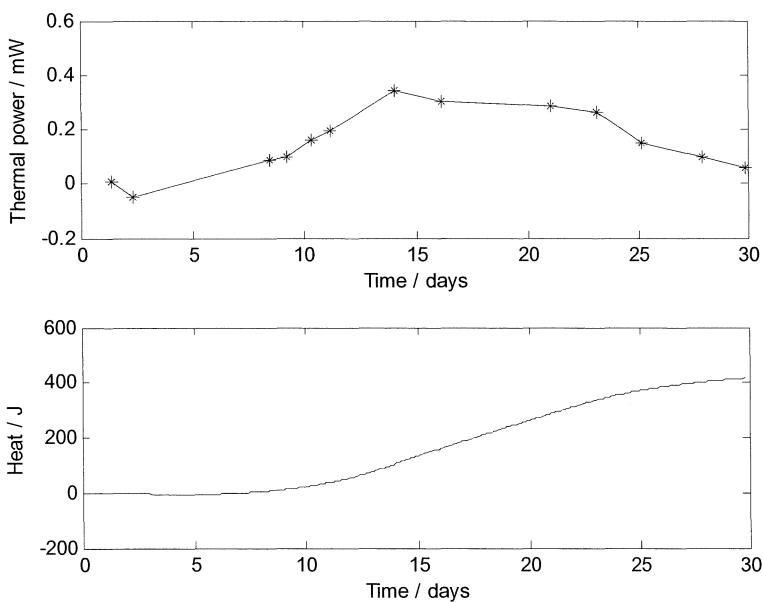
Figure 27: S. lacrymans (sample No. 31) thermal activities on MEA and the total heat production calculated by integrating the linearly interpolated top curve
