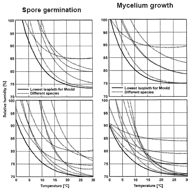
Figure 17: Isopleths for spore germination and mycelia growth of mould fungi and the Lowest Isopleth for Mould (LIM) resulting from that (Sedlbauer 2001)
