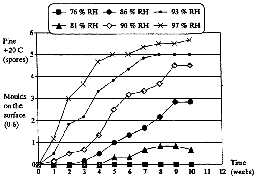
Figure 16: Mould growth on pine sapwood at temperature of 20°C (inoculated with spores) (Viitanen 1996)
