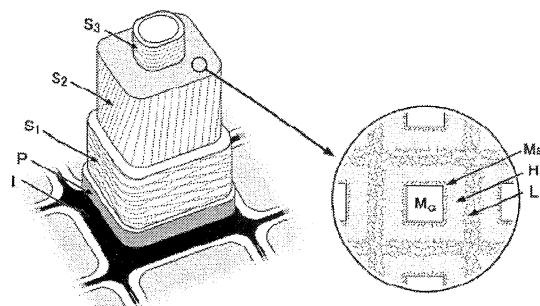
Figure 6: Microstructure of wood cell wall: (I) intercellular layer; (P) primary wall; (S1) outer layer of secondary wall; (S2) middle layer of secondary wall; (S3) inner layer of secondary wall; (Mc) crystalline region of microfibril; (Ma) amorphous region of microfibril; (H) hemicellulose; (L) lignin. (Nakano 2003)
