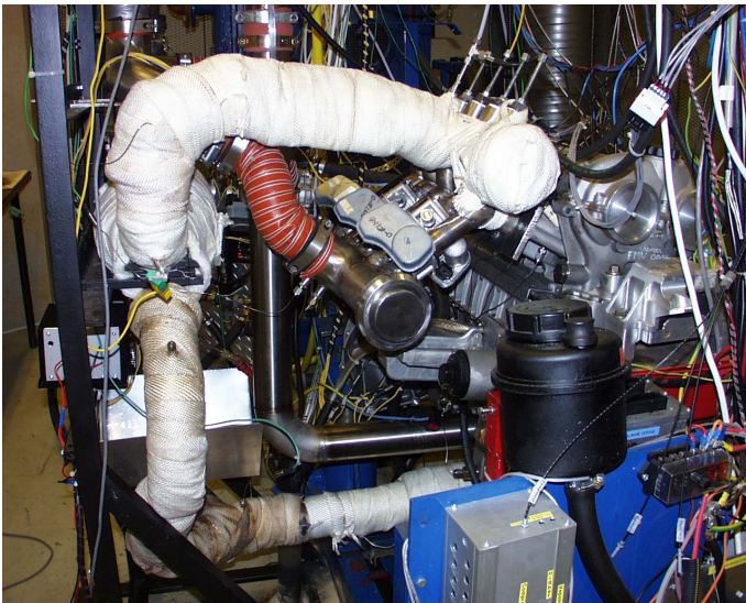
Figure 3 SVC engine with cylinder individual FTM system.
