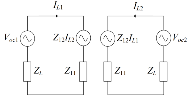
Fig. 1. Equivalent circuit for receive end.
