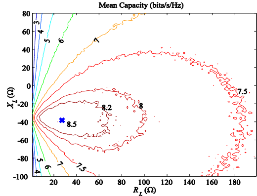
Fig. 10. Mean capacity for (\phi_0, \sigma) = (90^\circ, 40.6^\circ) and d = 0.1\lambda .
