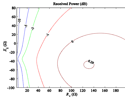
Fig. 5. Received power for (\phi_0, \sigma) = (0^\circ, 20.6^\circ) and d = 0.1\lambda .
