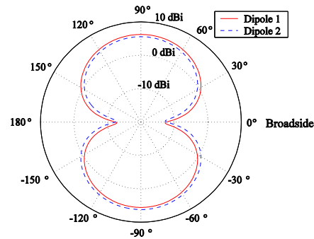
Fig. 3. Dipole antenna patterns with Z_L = 1.53 - j18.73\Omega at d = 0.05\lambda .
