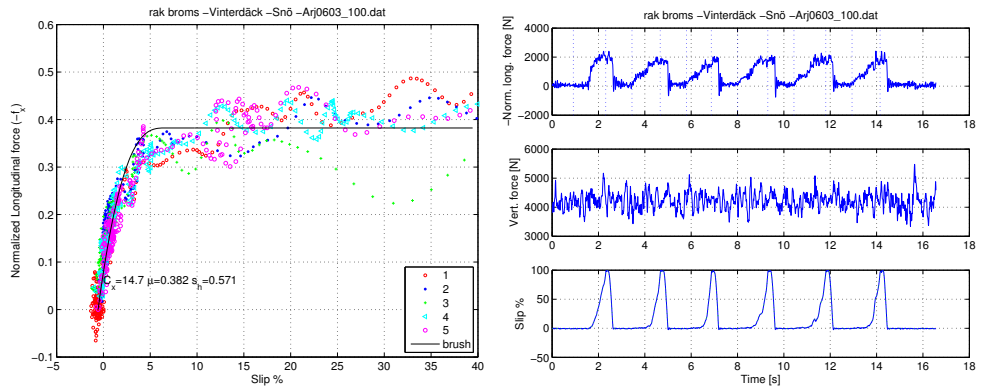
Figure 4 Results from braking test with winter tire on snow. Vertical load 4 kN.
