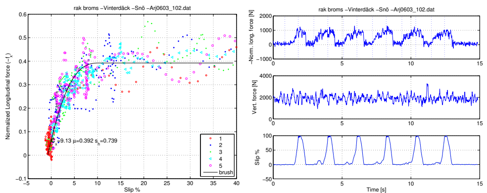
Figure 5 Results from braking test with winter tire on snow. Vertical load 2 kN
