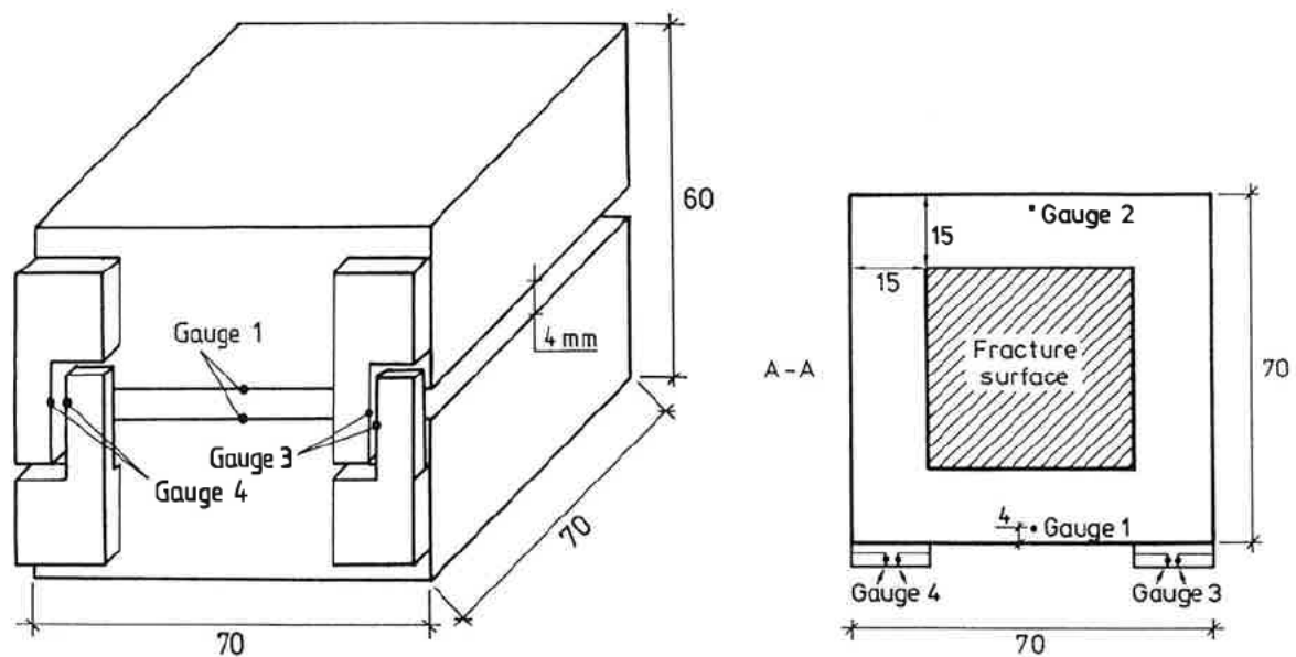
Fig. 3.22. Specimen geometry and locations of the clip gauges, in mm.
