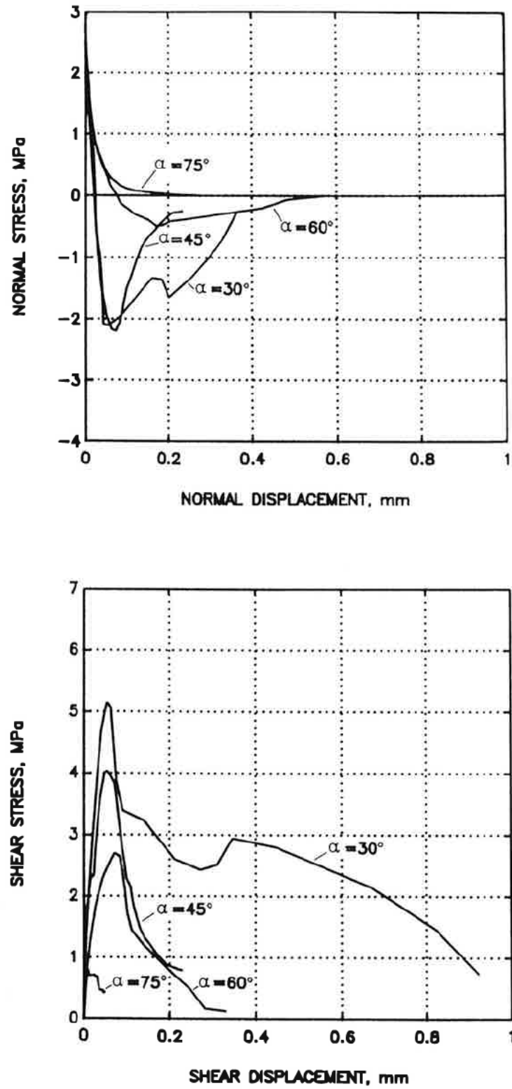
Fig. 4.14. Results of tests ( \sigma -w and \tau - \delta curves) on wet concrete specimens at the age of 28 days, linear paths.
