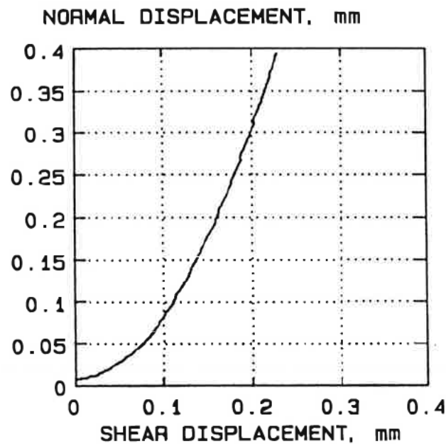
Fig. 4.9. Test with inverted parabolic displacement path ( w=7\delta^2 ).
