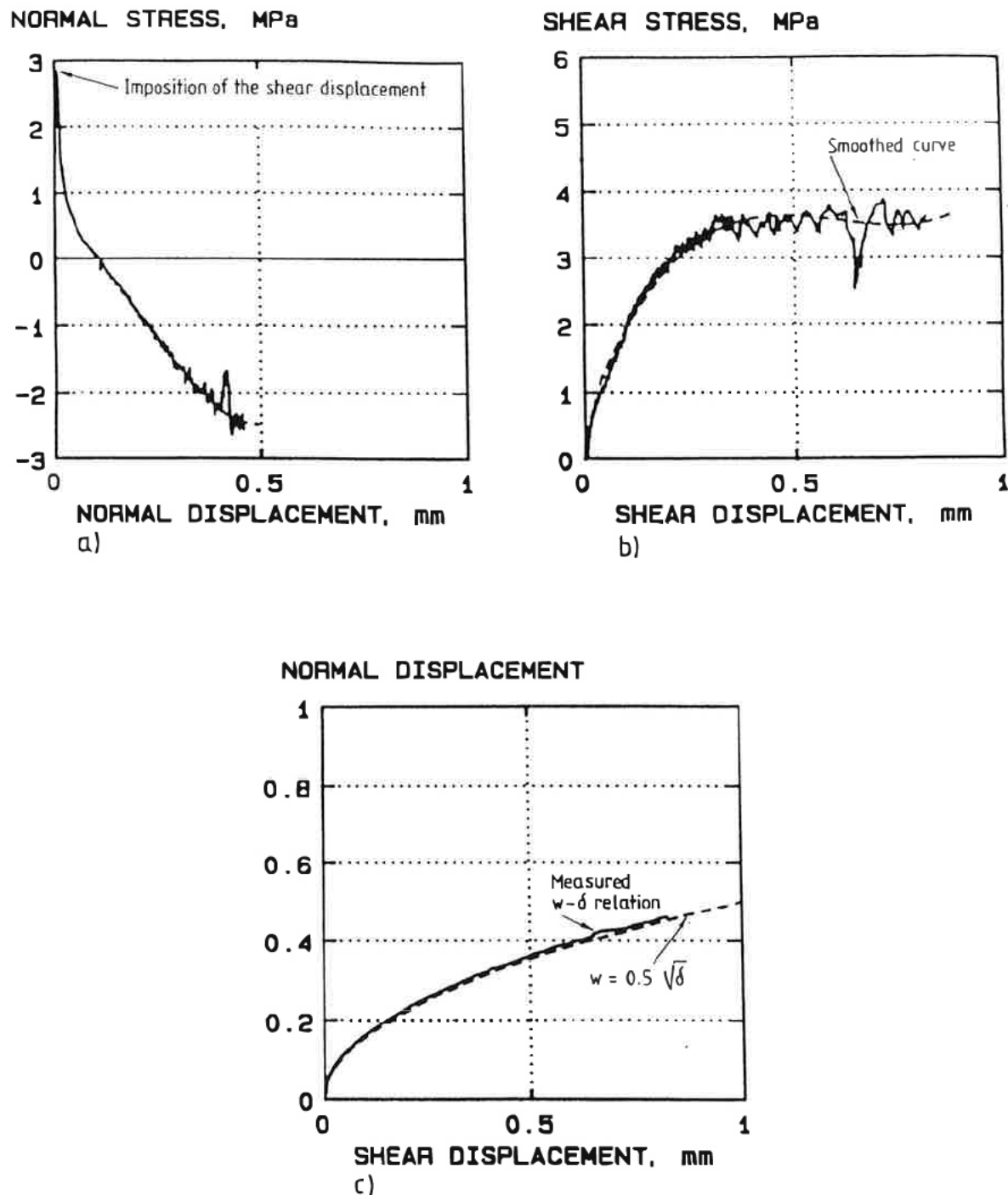
Fig. 4.2. Output of combined normal- and shear- displacement test. Parabolic path ( \beta=0.5 \text{ mm}^{1/2} ).
