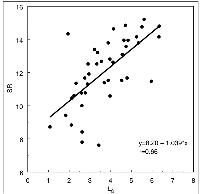
Figure 8. Relationship between L_G and SR for the deciduous plots ( n = 42 ).
