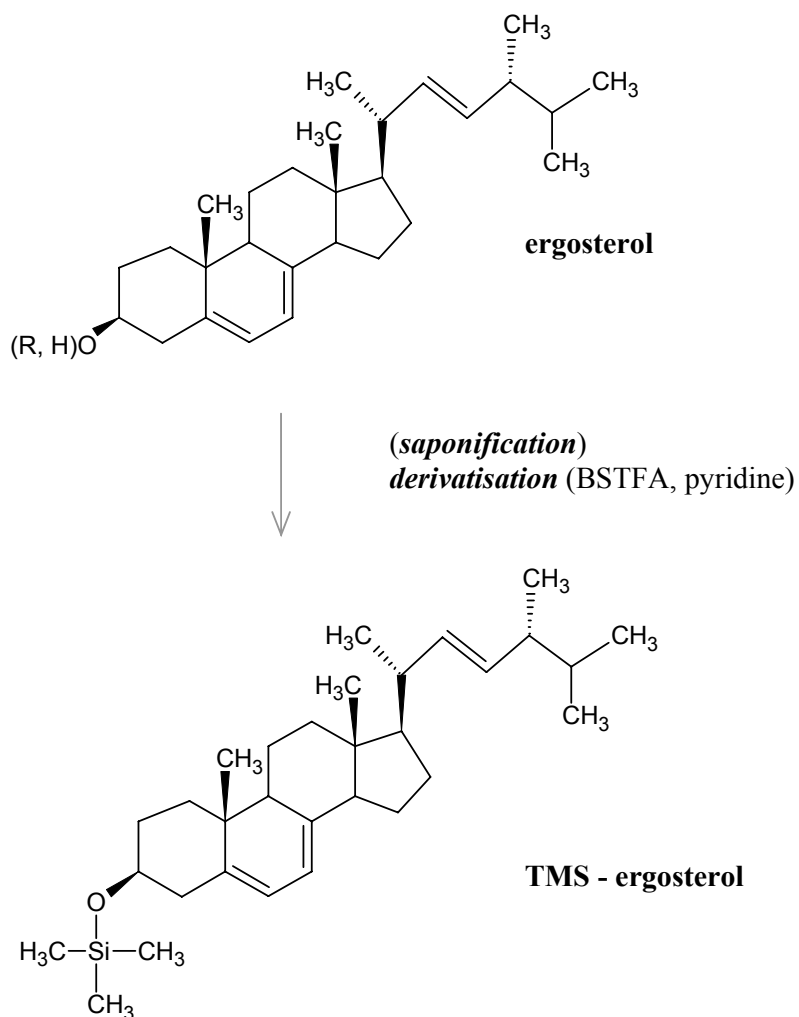
Figure 7. TMS derivatisation of ergosterol.
