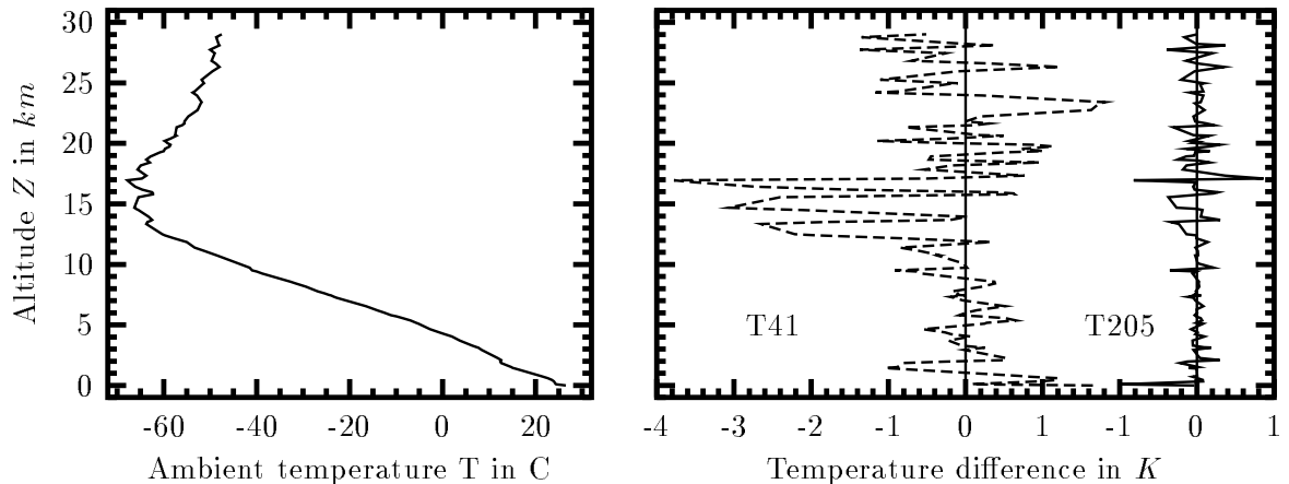
Fig. 7: This figure shows the temperature profile from the Sydney PTU sonde 99100915.syd (left panel). Interpolation errors are introduced if simple routines are used to map the sonde data onto the 41 standard altitudes (T41) normally handed to FSCATM. These errors are reduced significantly if the data is sampled at a much higher frequency (T205) as has become possible with the latest version of FSCATM (right panel).
