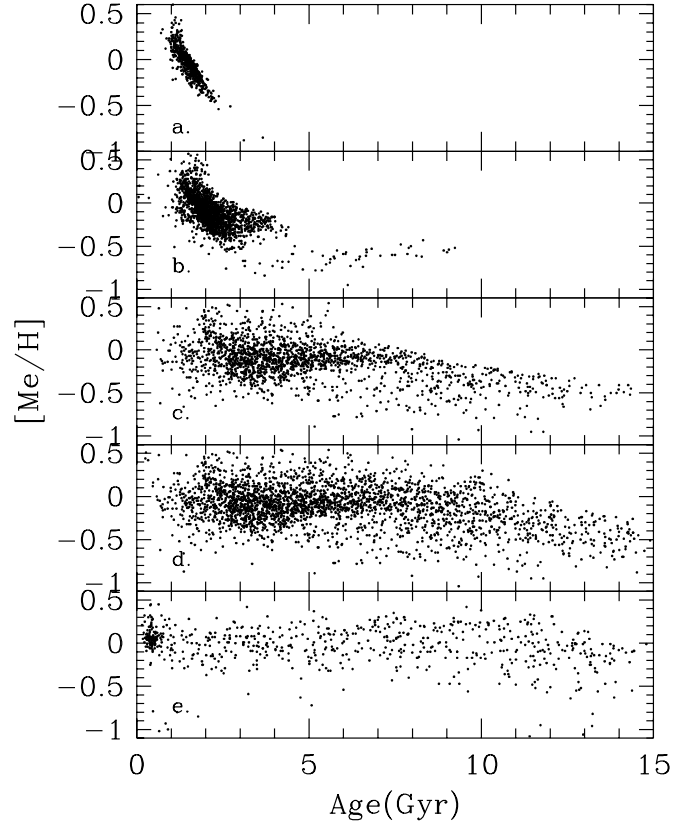
Fig. 13. Age-metallicity plots of different sub-samples from Fig. 10 and Fig. 12. a) Stars with \log T_{\text{eff}} > 3.83 , b) stars with 3.83 \geq \log T_{\text{eff}} > 3.8 , c) stars with 3.8 \geq \log T_{\text{eff}} > 3.77 , d) stars with 3.75 \geq \log T_{\text{eff}} > 3.7 , e) stars with 3.65 \geq \log T_{\text{eff}} . For clarity we only show [\text{Me}/\text{H}] > -1 . All stars have, as before, M_V < 4.4 and \sigma_\tau/\tau_{\text{mean}} \leq 0.5 and n \geq 2 .
