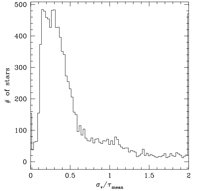
Fig. 3. Histogram of \sigma_\tau/\tau_{\text{mean}} for all stars in the full sample, excluding the 253 stars that have no good fit. See the text for explanation of \sigma_\tau and \tau_{\text{mean}} .
