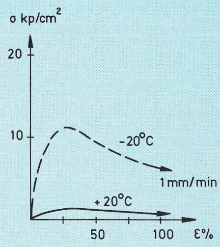
Akrylatfogmassa
