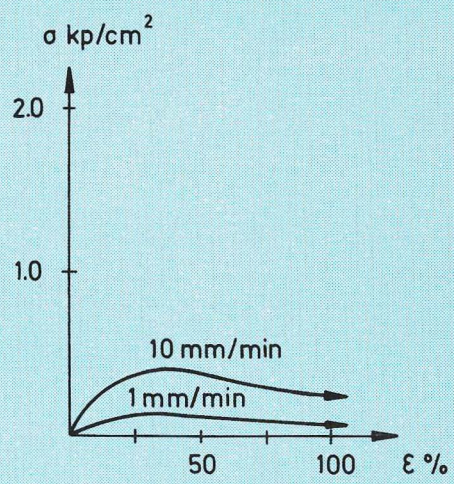
Akrylatfogmassa
