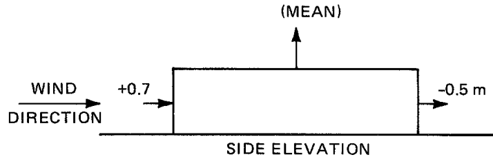
Figure 10.2 Square coefficients for an isolated, low, square building [ The SFPA Handbook of Fire Protection Engineering ].
