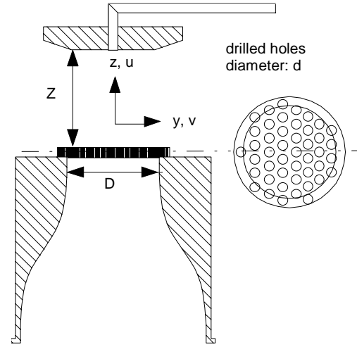
Figure 3. Test section.
